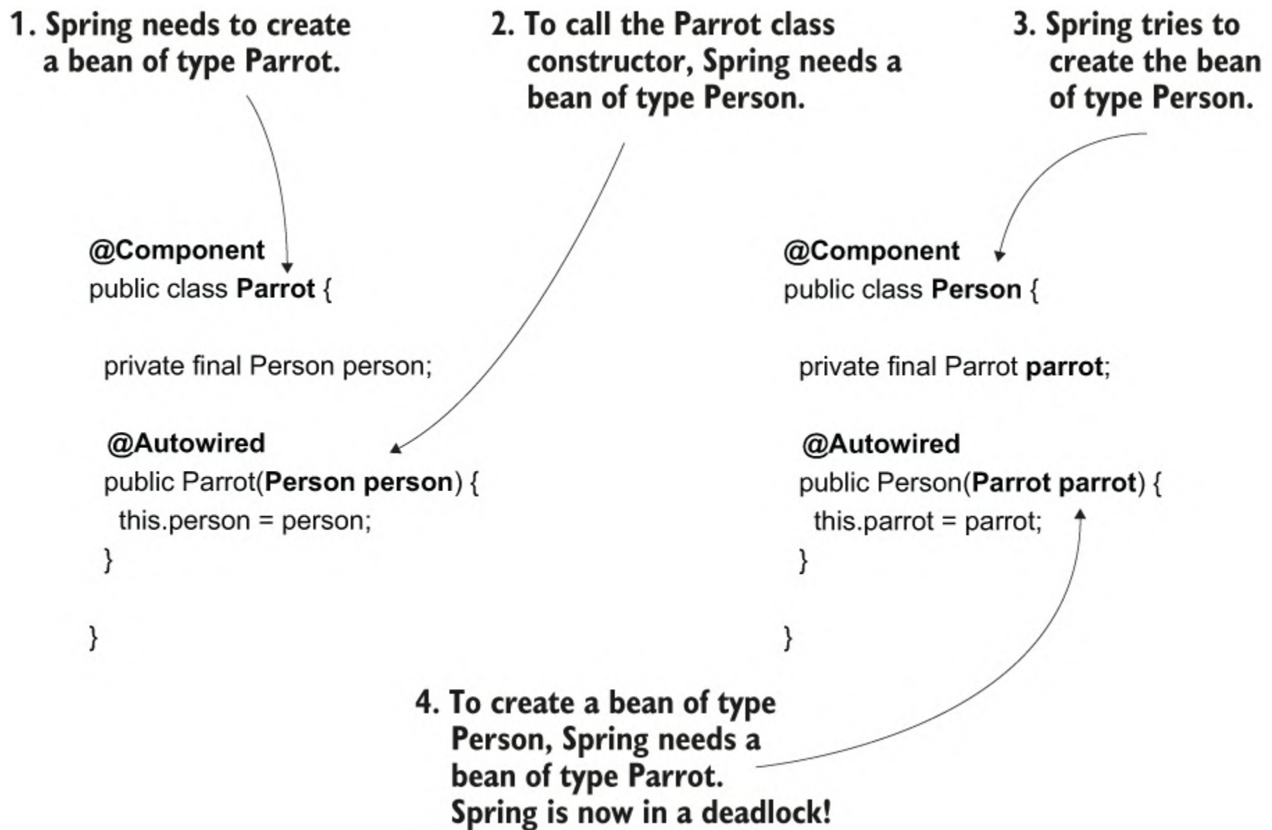
Figure 3.11 A circular dependency. Spring needs to create a bean of type Parrot . But because Parrot has as a dependency a Person , Spring needs first to create a Person . However, to create a Person , Spring already needs to have built a Parrot . Spring is now in a deadlock. It cannot create a Parrot because it needs a Person , and it cannot create a Person because it needs a Parrot .
