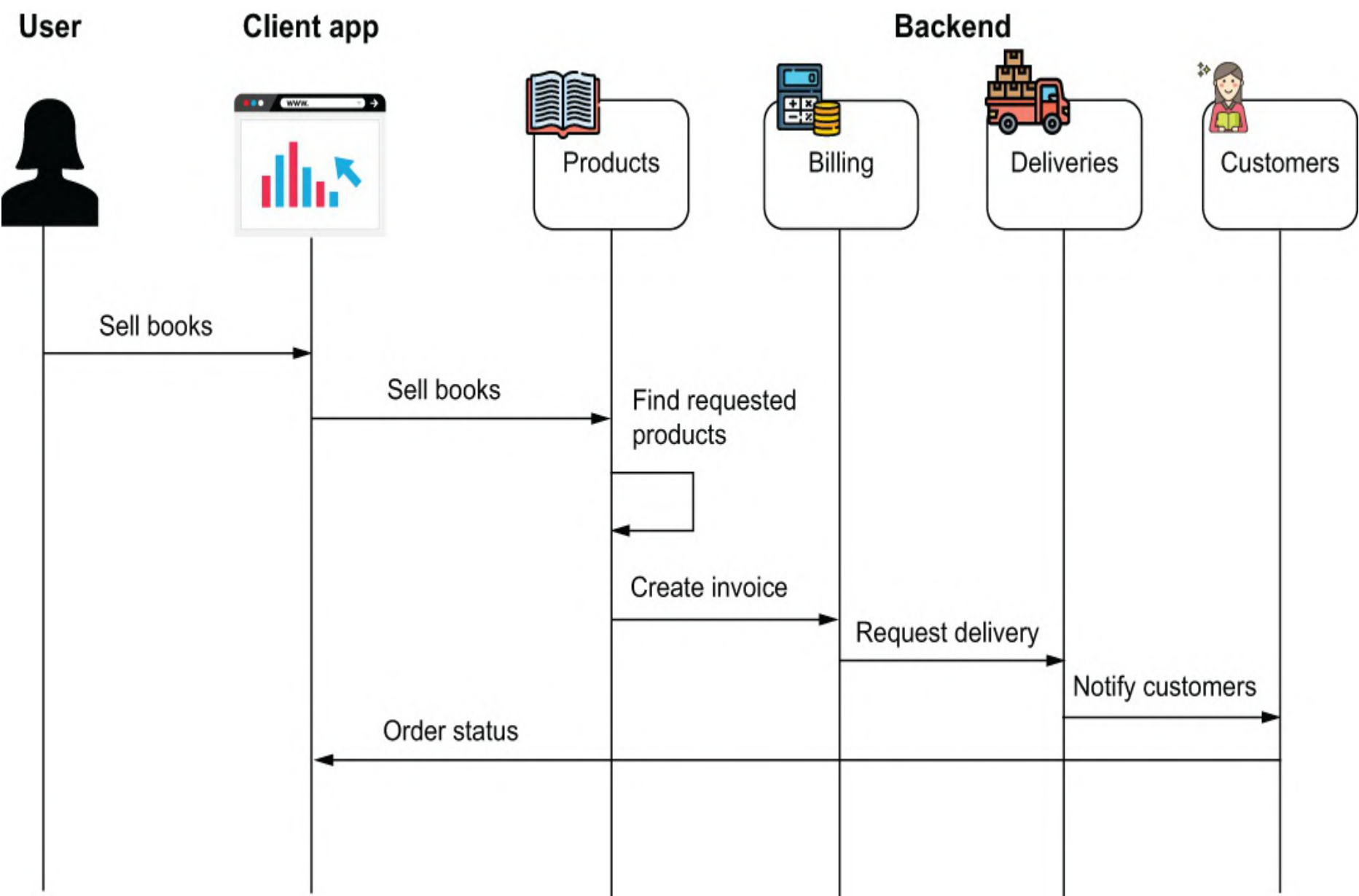
Figure A.2 An example of business flow. The user wants to sell books. The client app sends the request to the backend. Each responsibility of the backend has a role in the entire flow. The functionalities communicate with each other to complete the business flow. In the end, the client app receives the status of the order
