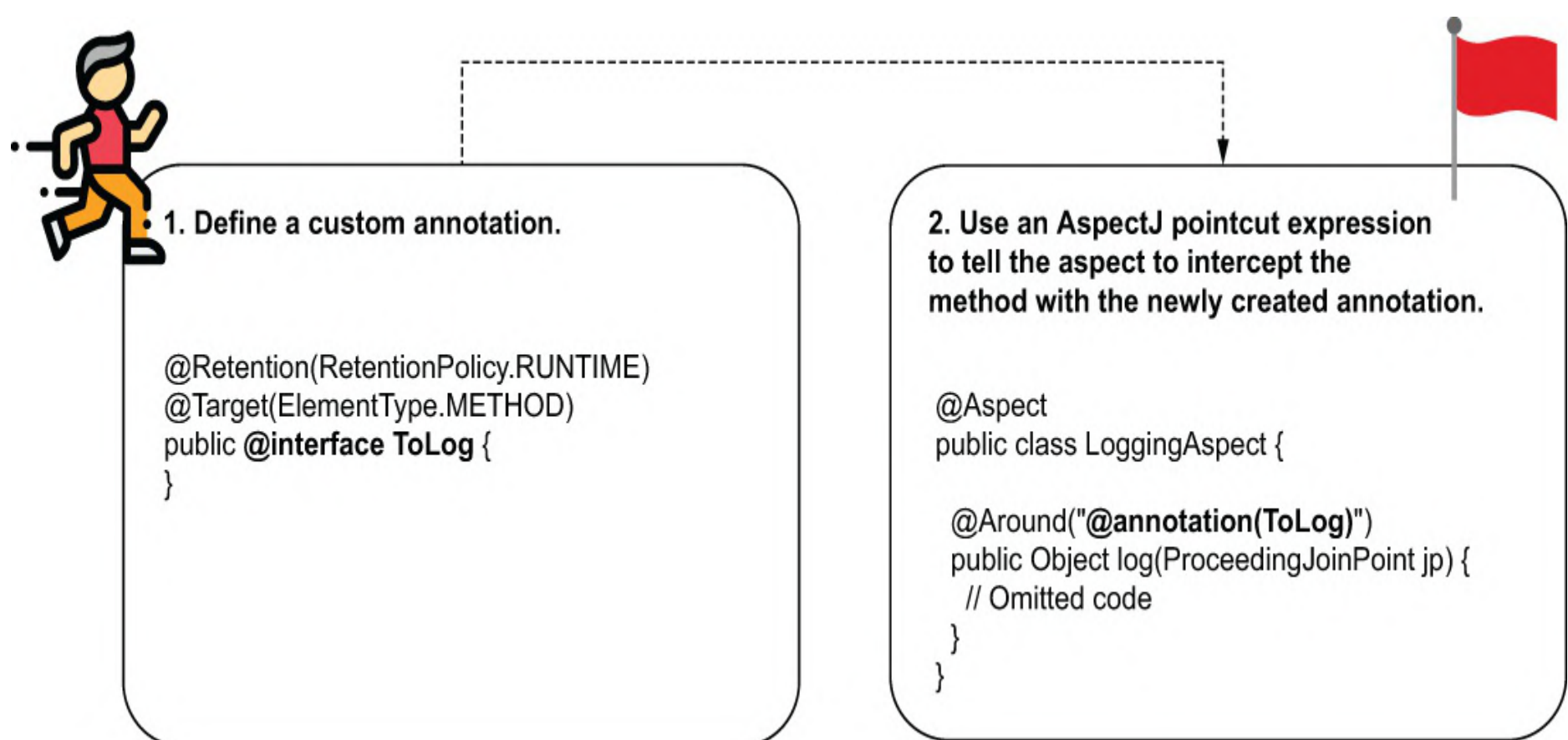
Figure 6.12 The steps for intercepted annotated methods. You need to create a custom annotation you want to use to annotate the methods your aspect needs to intercept. Then you use a different AspectJ pointcut expression to configure the aspect to intercept the methods annotated with the custom annotation you created.
