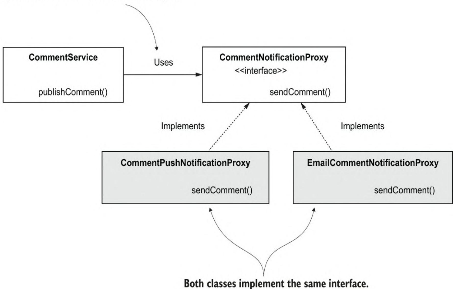
Figure 4.9 Sometimes, in real-world scenarios, we have multiple implementations of the same interface. When using dependency injection on the interface, you need to instruct Spring which is the implementation it should inject.
