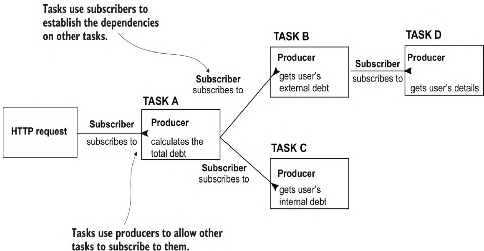
Figure 11.10 In a reactive app, the steps become tasks. Each task marks its dependencies on other tasks and allows other tasks to depend on them. Threads are free to execute any task.
