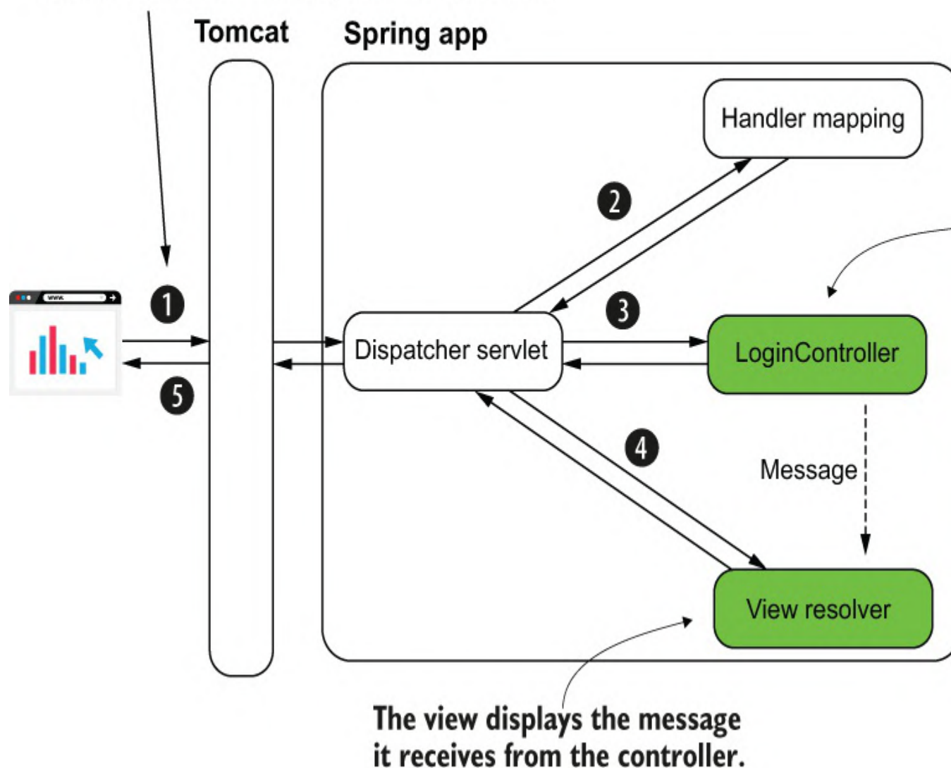
Figure 9.3 We need to implement the controller and the view. In the controller, we implement an action that finds out if the credentials sent in the login request are valid. The controller sends a message to the view, and the view displays this message.
