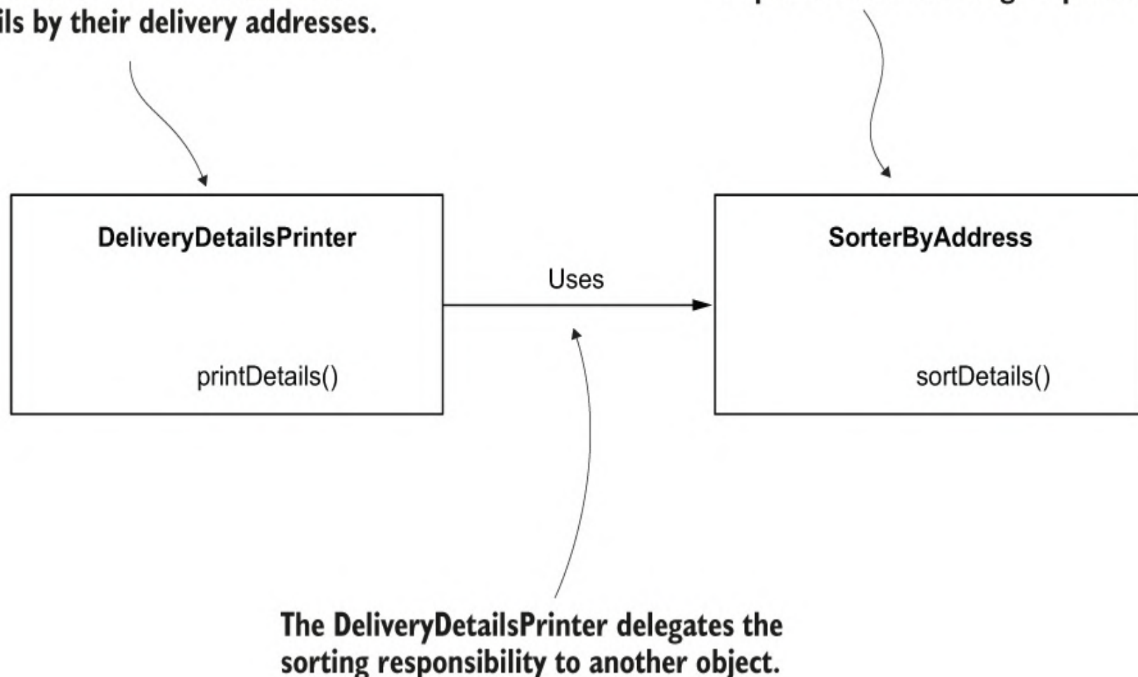
Figure 4.1 The DeliveryDetailsPrinter object delegates the responsibility of sorting the delivery details by the delivery addresses to another object named SorterByAddress .
