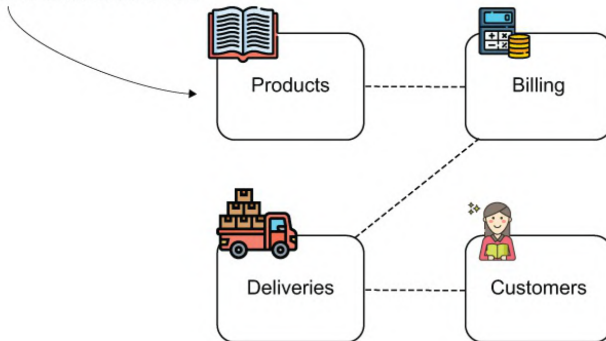
Figure A.5 In a SOA, each feature is an independent process. This way, you can decide to scale just the features that need more resources.
