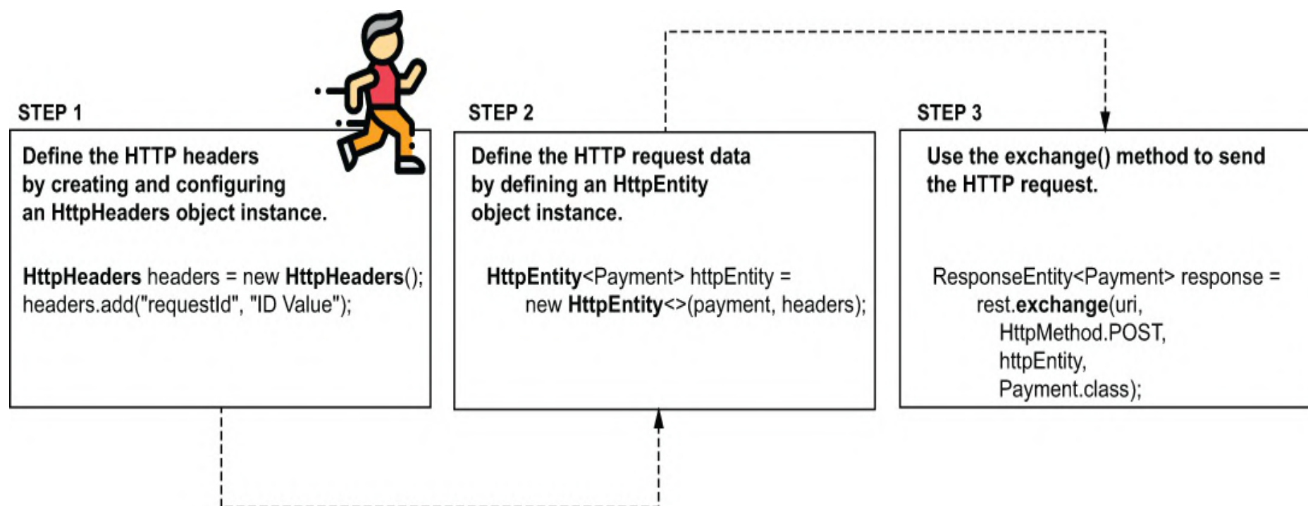
Figure 11.6 To define a more complex HTTP request, you have to use the HttpHeaders class to define the headers, then the HttpEntity class to represent the full request data. Once you defined the data on the request, you call the exchange() method to send it.
