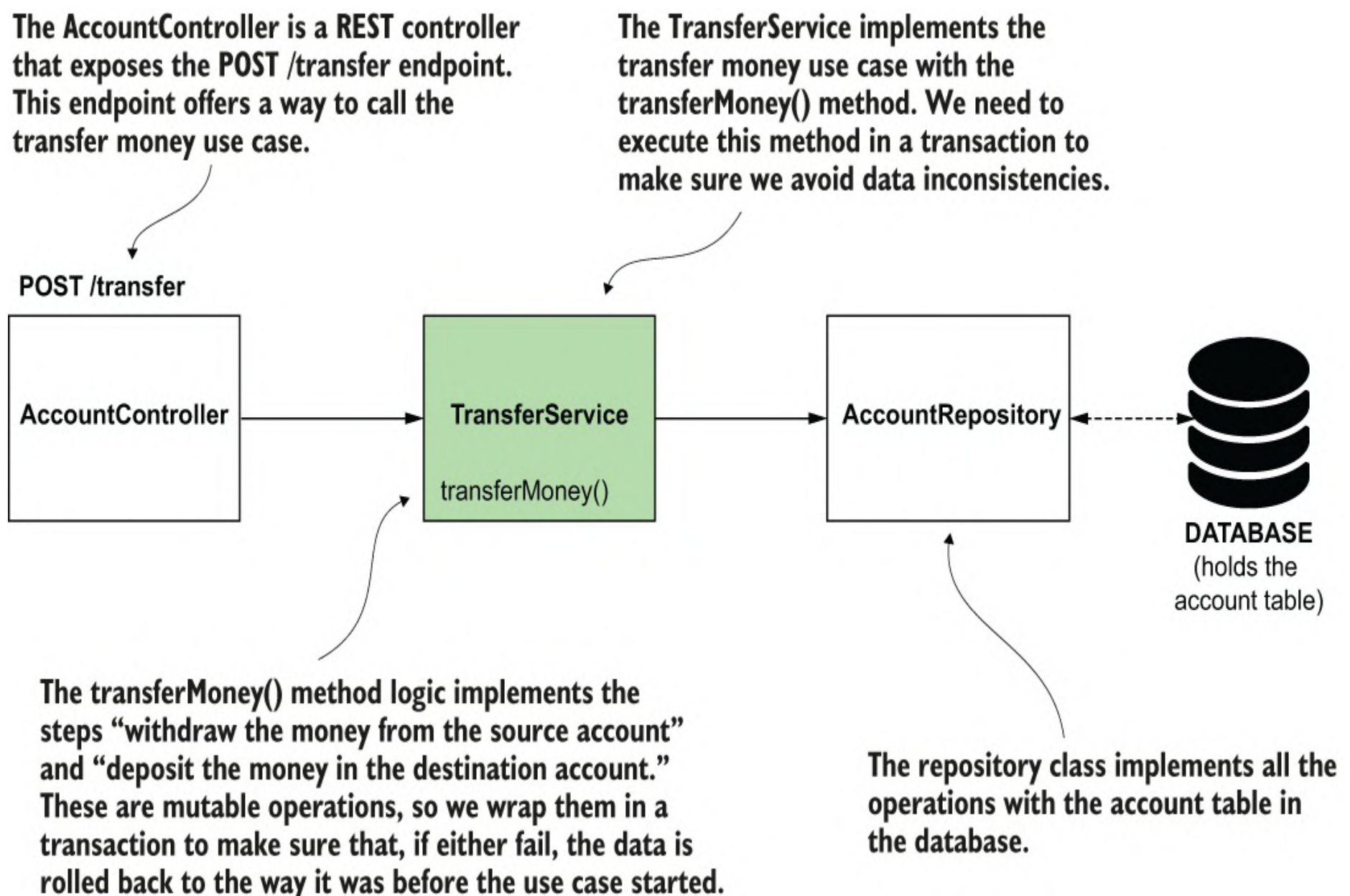
Figure 13.6 We implement the transfer money use case in a service class and expose this service method through a REST endpoint. The service method uses a repository to access the data in the database and change it. The service method (which implements the business logic) must be wrapped in a transaction to avoid data inconsistencies if problems occur during the method execution.
