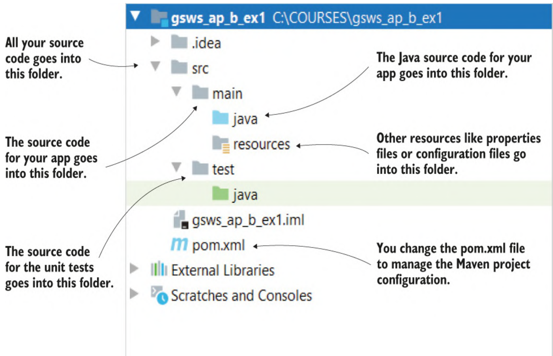
Figure 2.3 How a Maven project is organized. Inside the src folder, we add everything that belongs to the app: the application's source code goes into the main folder, and the source code for the unit tests goes into the test folder. In the pom.xml file we write configurations for the Maven project (in our examples we'll primarily use it to define the dependencies).
