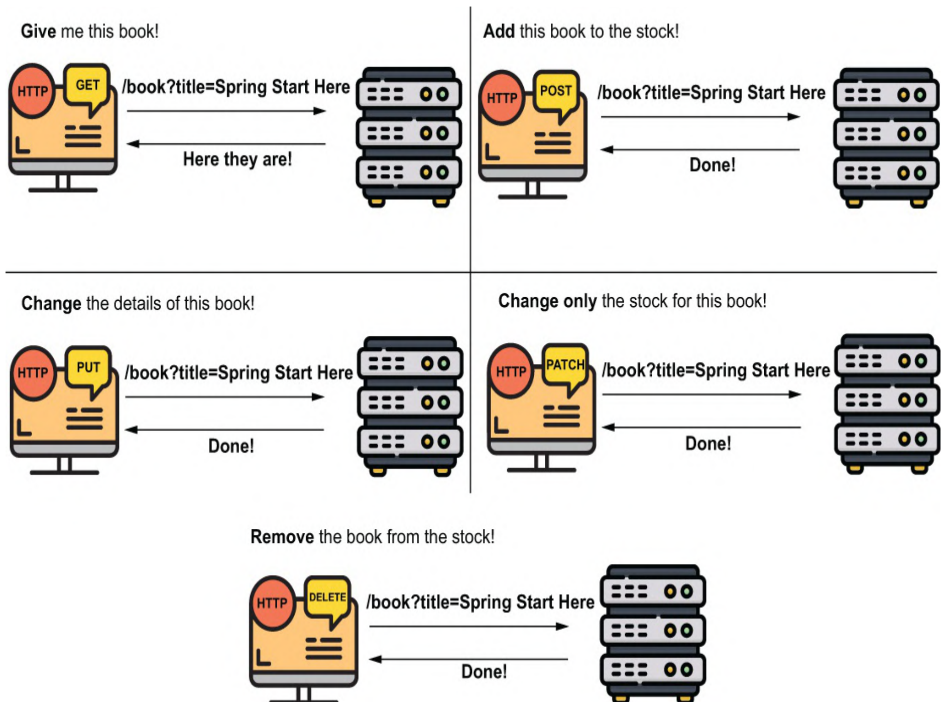
Figure 8.9 The basic HTTP methods. You use GET for retrieving data, POST for adding data, PUT for changing a record, PATCH for changing a part of the record, and DELETE to remove data. The client must use the appropriate HTTP method to express the action executed by a specific request.
