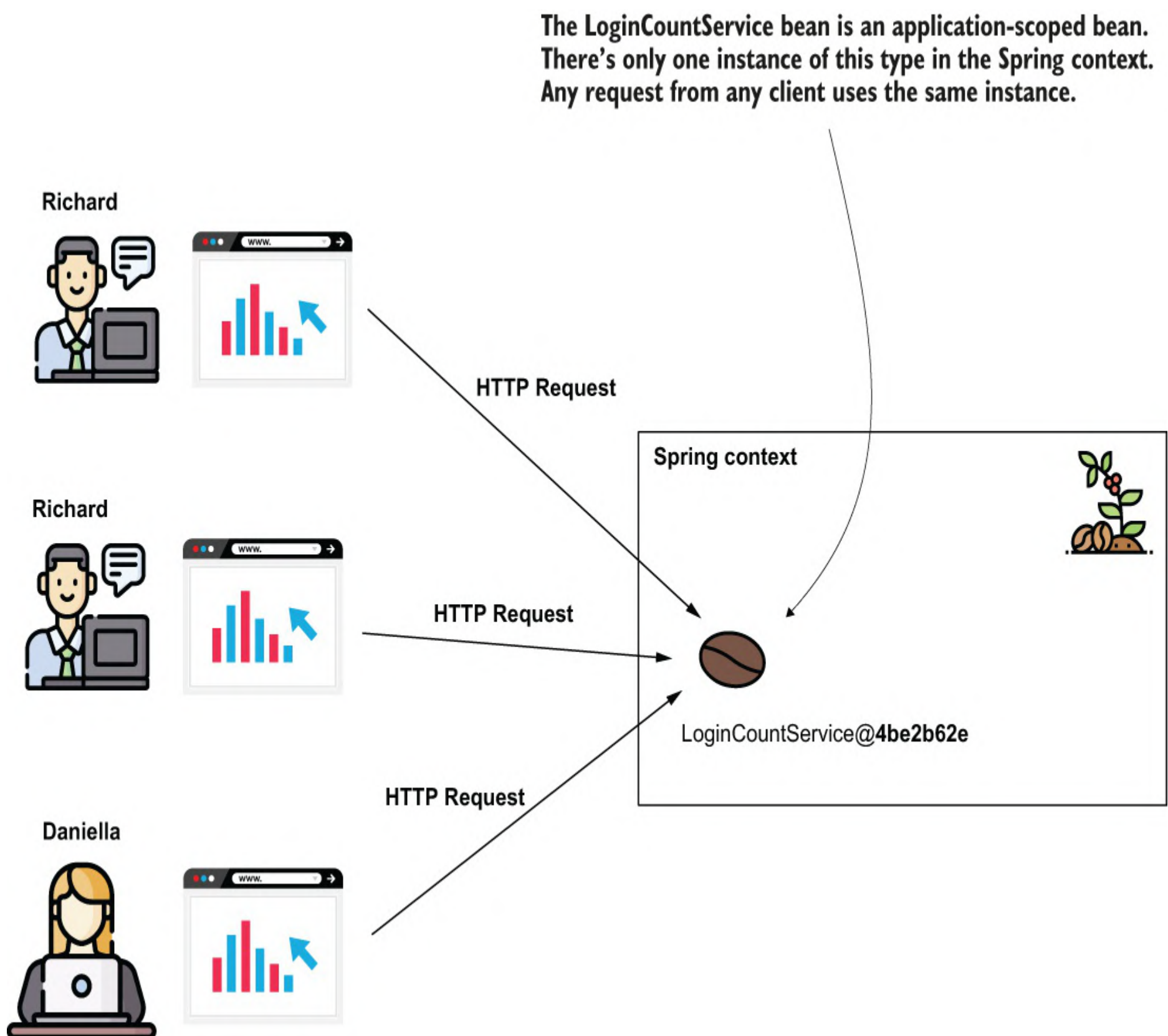
Figure 9.14 Understanding the application scope in a Spring web app. The instance of an application-scoped bean is shared by all the HTTP requests from all clients. The Spring context provides only one instance of the bean's type, used by anyone who needs it.
