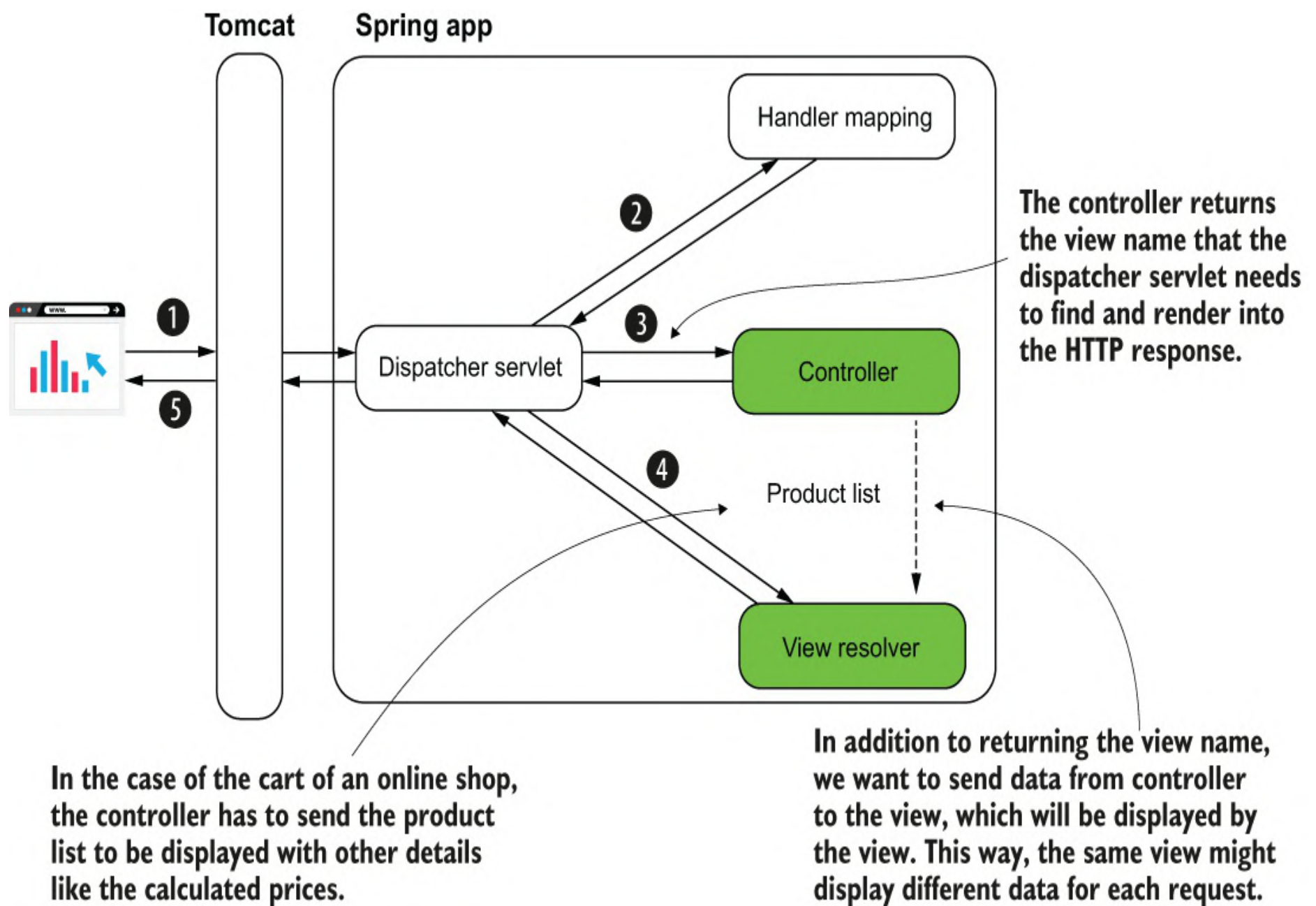
Figure 8.3 The Spring MVC flow. To define a dynamic view, the controller needs to send data to the view. The data the controller sends can be different for each request. For example, in an online shop's cart functionality, the controller initially sends a list of one product to the view. After the user adds more products, the list the controller sends contains all the products in the cart. The same view shows different information for these requests.
