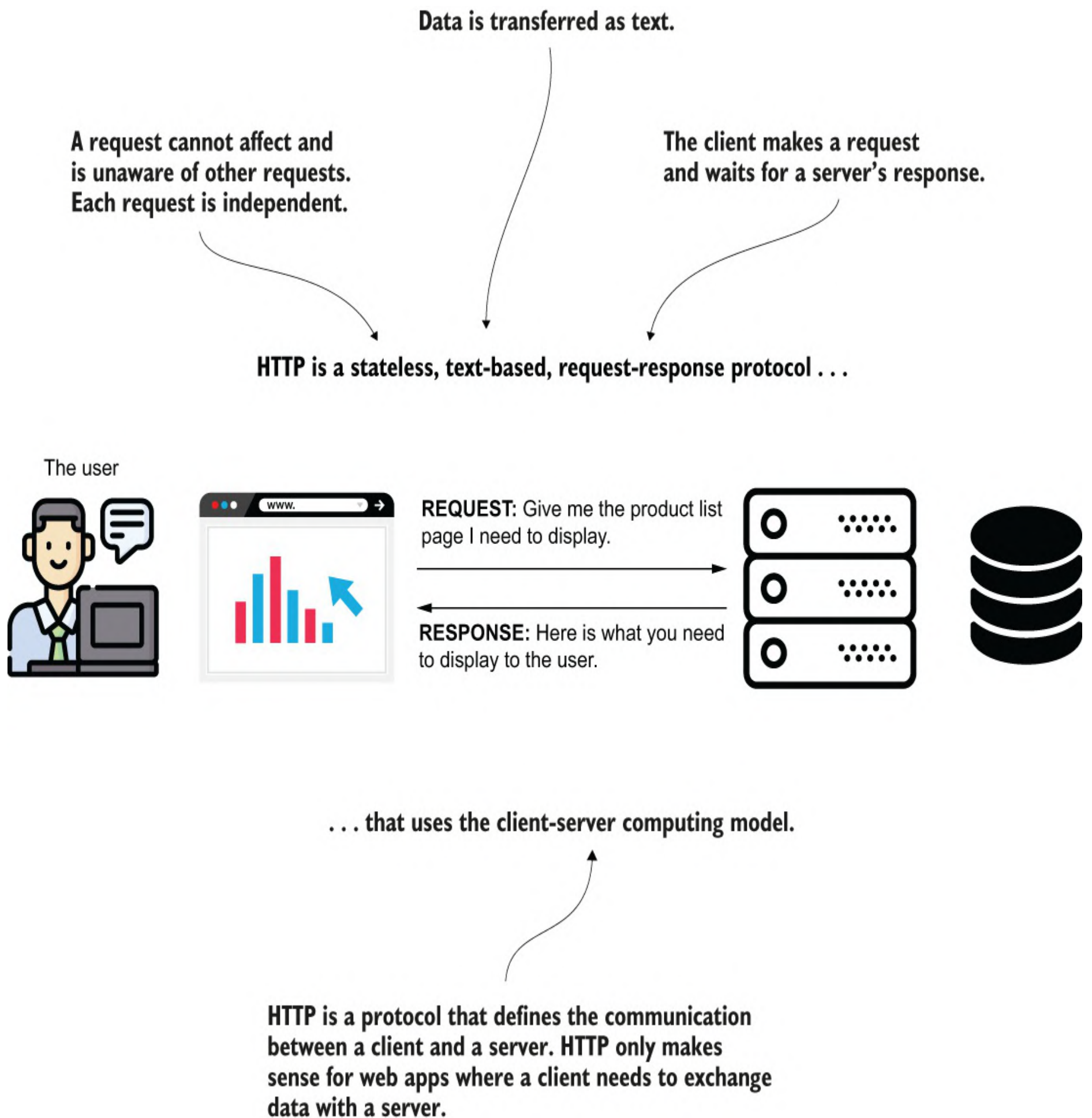
Figure C.1 HTTP is a protocol that describes how a client and a server talk. HTTP assumes a client makes a request, and the server responds. The protocol describes what the client's request and the server's response look like. HTTP is stateless, meaning the requests are independent of one another, and text-based, which means the information is exchanged as plain text.
