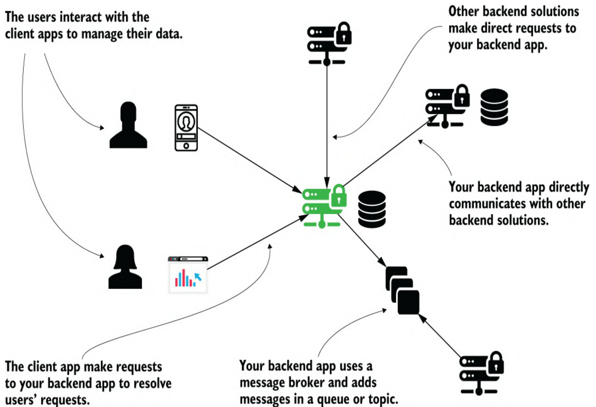
Figure 1.5 A backend app interacts in several ways with other apps and uses databases to manage data. Usually, a backend app is complex and may require the use of various technologies. Frameworks simplify the implementation by providing tools you can use to implement the backend solution faster.
