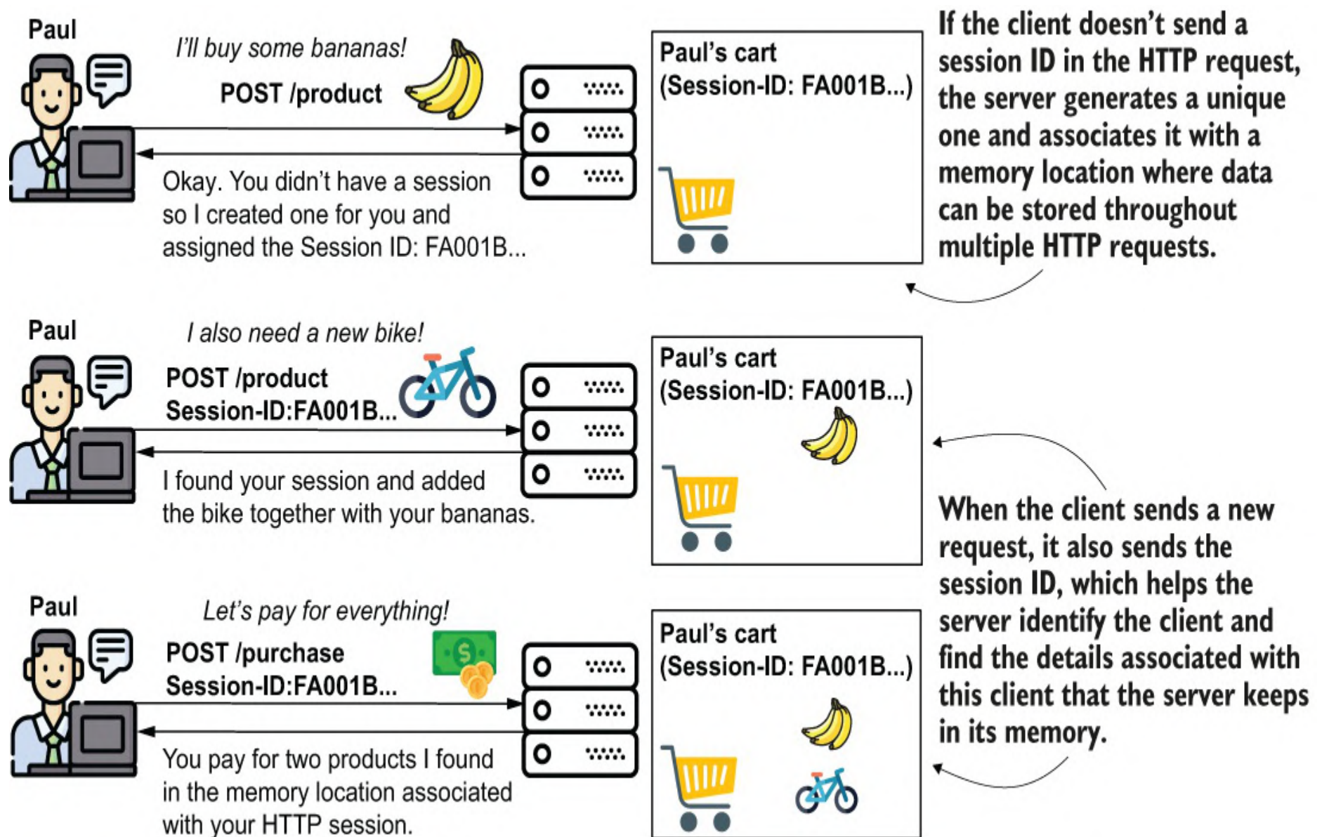
Figure C.4 The HTTP session mechanism. The server identifies the client with a unique session ID it generates. The client sends the session ID in the next requests, so the backend app knows which memory location it reserved earlier for the client.
