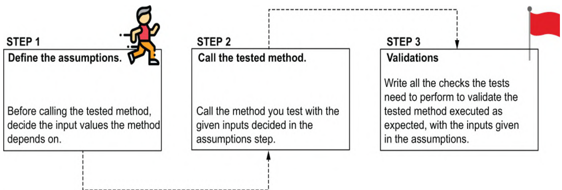
Figure 15.5 The steps for writing a unit test. Write the assumptions by defining the method inputs. Call the method with the defined assumptions and write the checks the tests need to perform to validate the method's behavior is correct.
