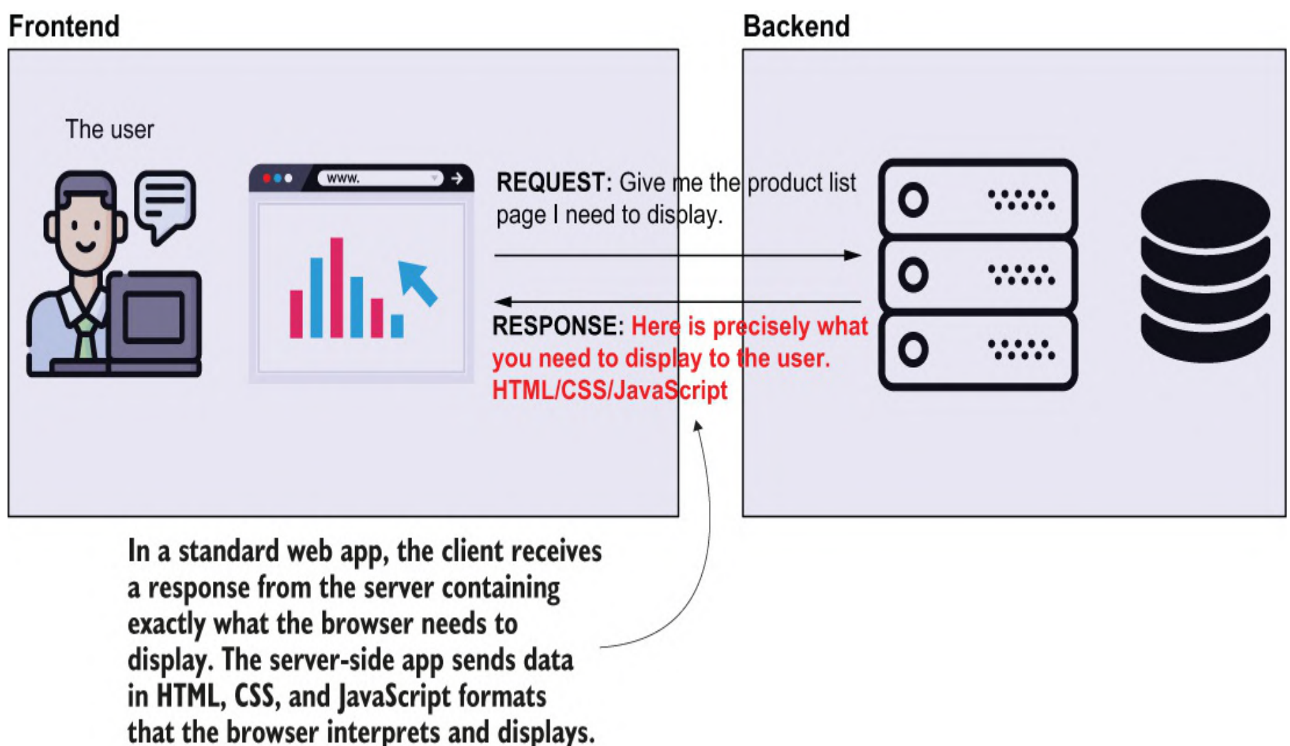
Figure 7.4 When a web app doesn't provide frontend-backend separation, the browser precisely displays what it gets from the server. The server gets requests from the browser, executes some logic, and then responds. In response, the backend provides content formatted as HTML, CSS, and other fashions that the browser interprets to display.
