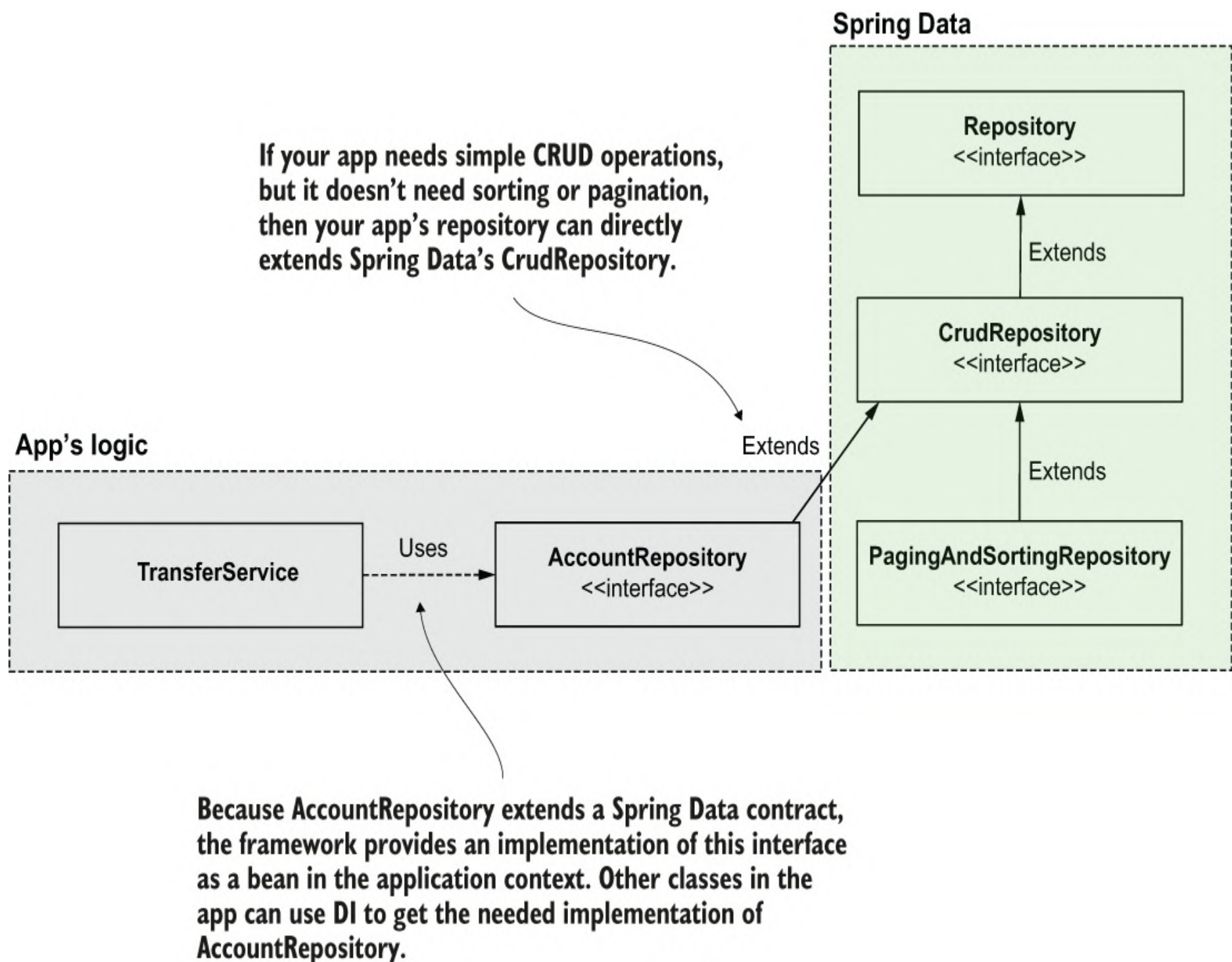
Figure 14.7 To create a Spring Data repository, you define an interface that extends one of the Spring Data contracts. For example, if your app only needs CRUD operations, the interface you define as a repository should extend the crudRepository interface. The app adds a bean that implements the contract you define to the Spring context, so any other app components that need to use it can simply inject it from the context.
