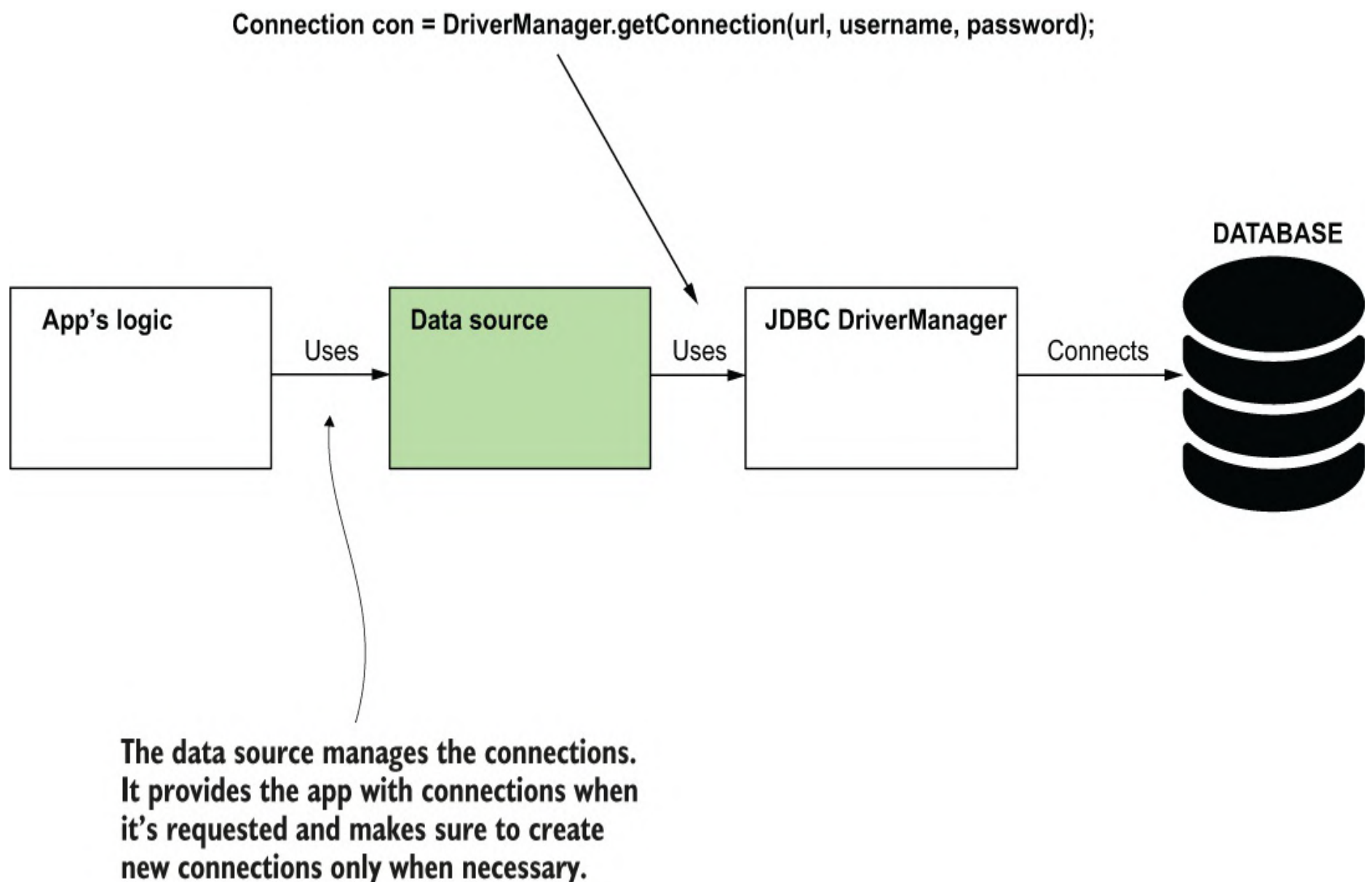
Figure 12.5 Adding a data source to the class design helps the app spare the time for unnecessary operations. The data source manages the connections, provides the app with connections when requested, and creates new connections only when needed.
