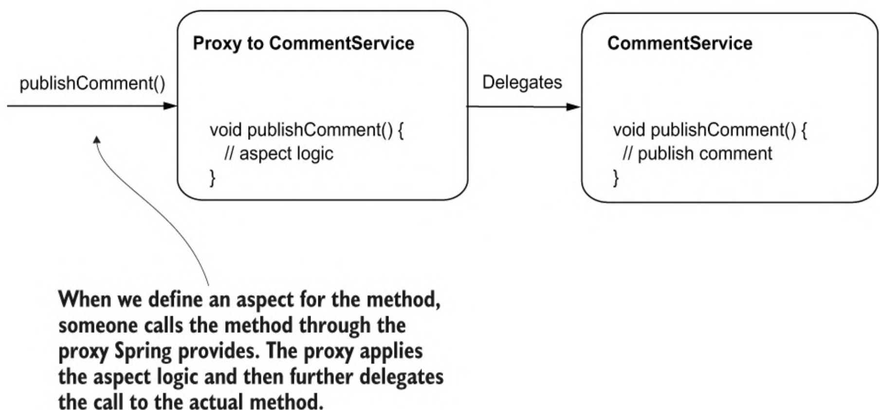
Figure 6.4 When a method isn't aspected, the call goes directly to that method. When we define an aspect for a method, the call goes through the proxy object. The proxy object applies the logic defined by the aspect and then delegates the call to the real method.
