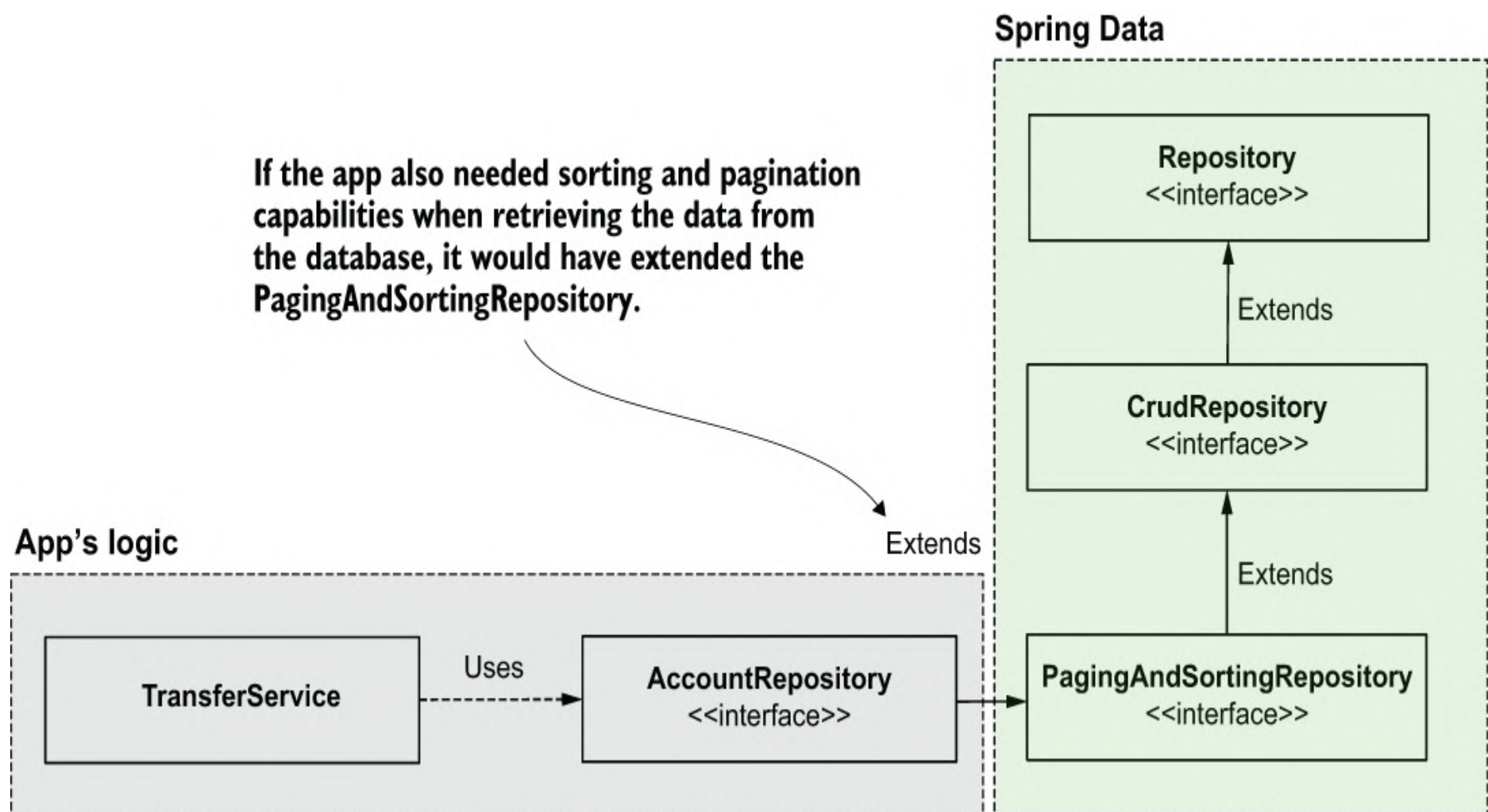
Figure 14.8 If the app needs sorting and pagination capabilities, it should extend a more particular contract. The app provides a bean that implements the contract, which can then be injected from any other component that needs to use it.
