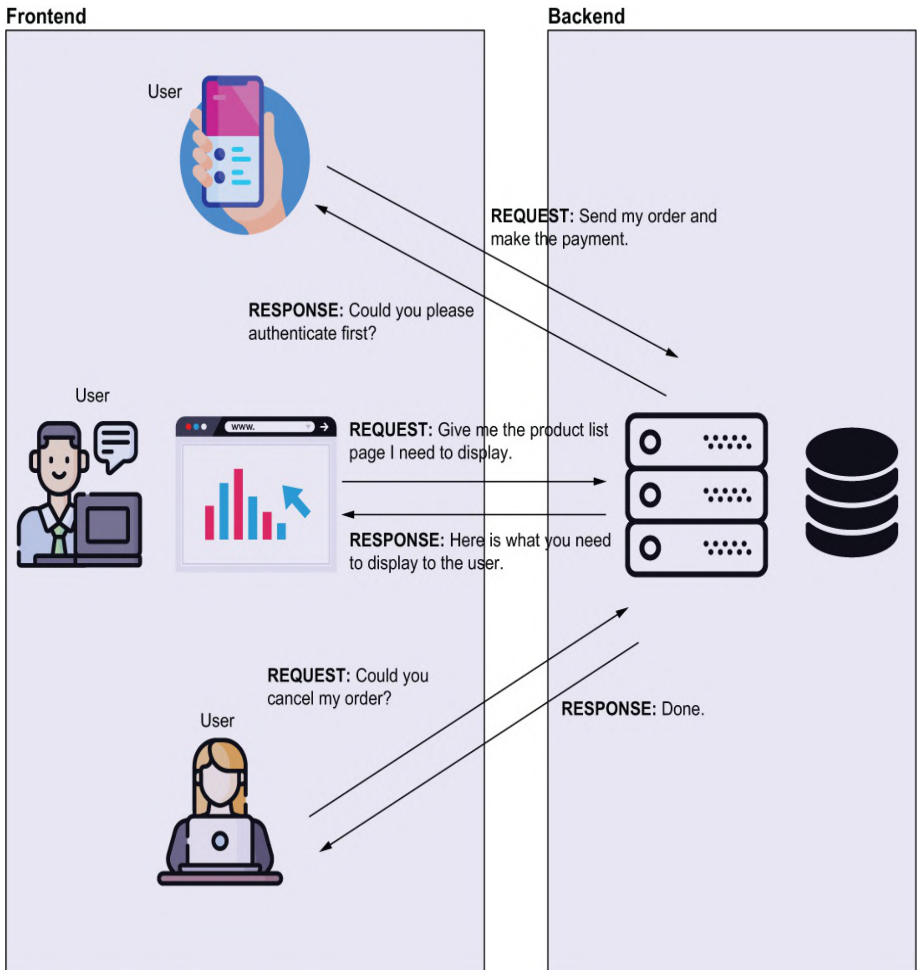
Figure 7.3 When discussing web apps, we refer to the client as being one instance, but keep in mind that multiple users access a browser and use the same web app concurrently. Each user makes their own requests on specific actions they need to execute. This is important because it means that some operations on the backend execute concurrently. If you write code that accesses and changes the same resource, your app might wrongly behave because of race condition scenarios.
