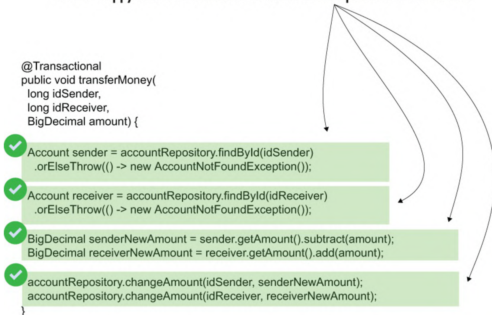
Figure 15.4 The happy flow: an execution for which no errors or exceptions are encountered. Usually, the happy flows are the first to write tests because they are the most obvious scenarios.
