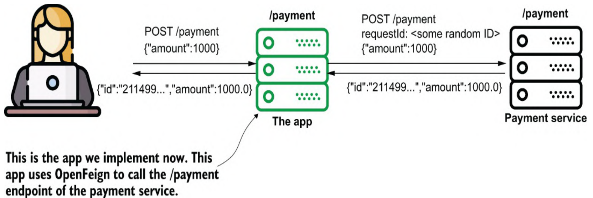
Figure 11.4 We now implement the app that consumes the /payment endpoint the payment service exposes. We use openFeign to implement the functionality that consumes the REST endpoint.
