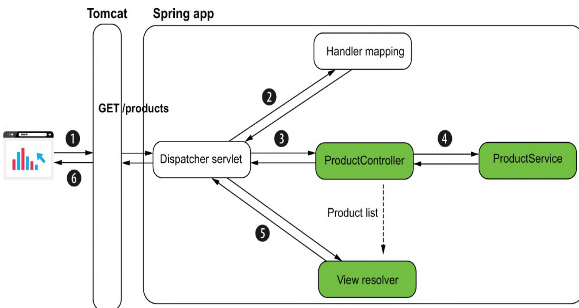
Figure 8.10 When calling /products with HTTP GET, the controller gets the product list from the service and sends it to the view. The HTTP response contains the HTML table with the products from the list.
