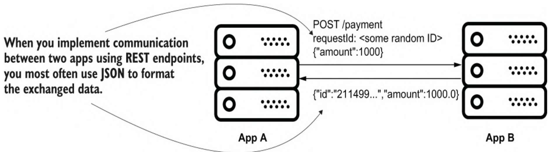
Figure D.1 When you implement business logic, it sometimes implies establishing communication between multiple apps. Most often, you use JSON to format the data the apps exchange. To implement and test your REST endpoints, you need to understand JSON.
