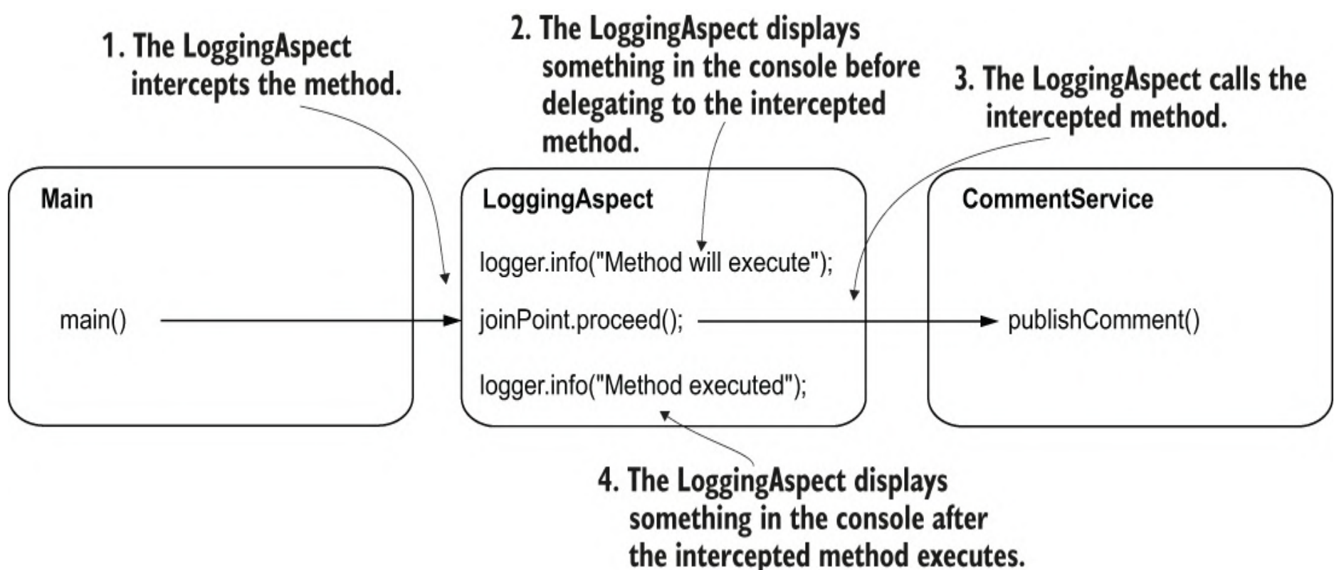
Figure 6.7 The aspect behavior. LoggingAspect wraps the method execution by displaying something before and after the method call. This way, you observe a simple implementation of an aspect.
