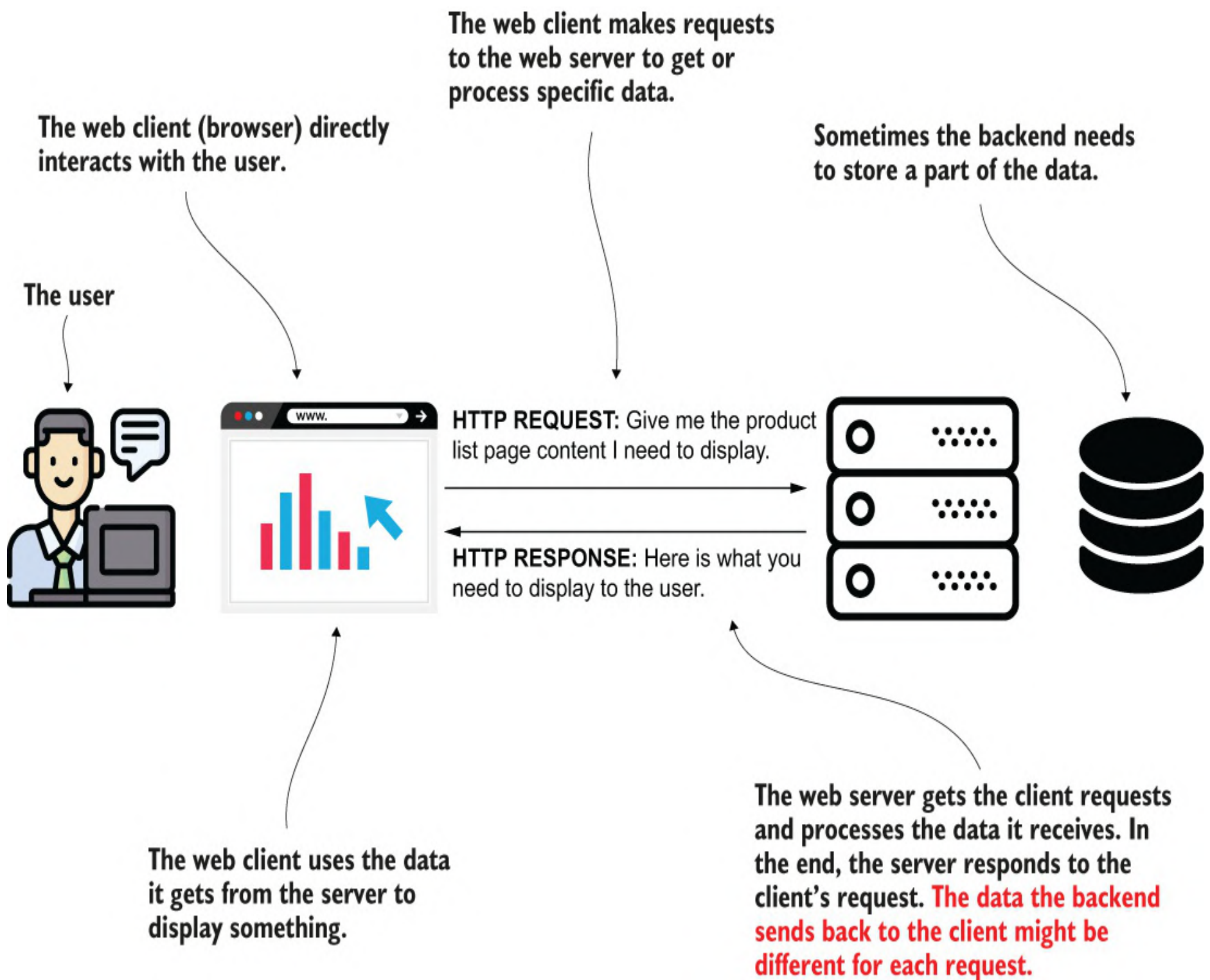
Figure 8.2 A client sends data through the HTTP request. The backend processes this data and builds a response to send back to the client. Depending on how the backend processed the data, different requests may result in other data displayed to the user.
