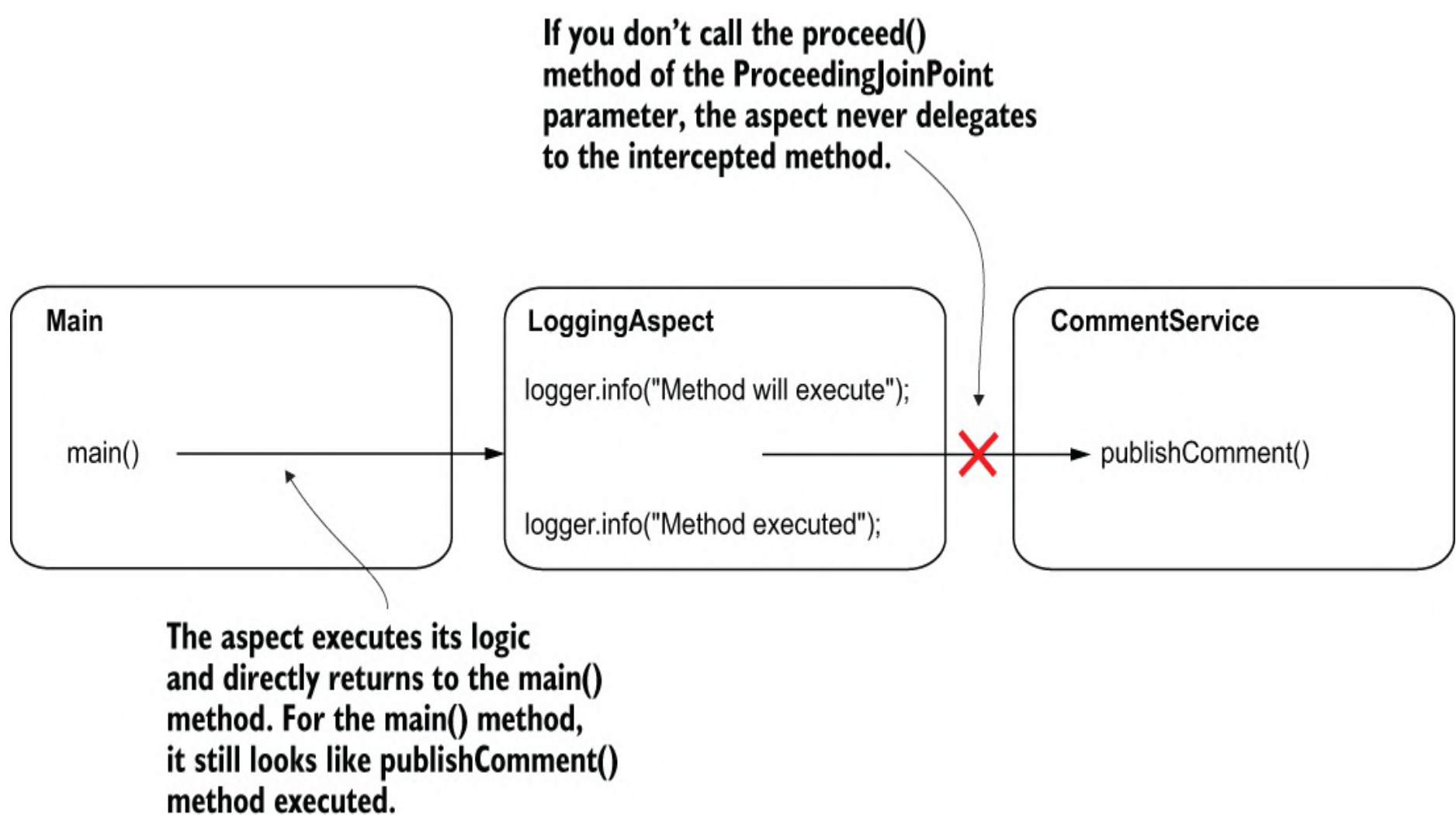
Figure 6.8 If you don't call the proceed() method of the ProceedingJoinPoint parameter of the aspect, the aspect never delegates further to the intercepted method. In this case, the aspect simply executes instead of the intercepted method. The caller of the method doesn't know that the real method is never executed.
