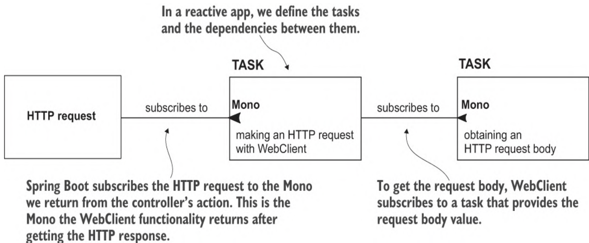
Figure 11.11 The tasks chain in a reactive app. When building a reactive web app, we define the tasks and the dependencies between them. The webFlux functionality initiating the HTTP request subscribes to the task we create through the producer the controller's action returns. In our case, this producer is the one we get by sending the HTTP request with webClient . For webClient to make the request, it subscribes to another task that provides the request body.
