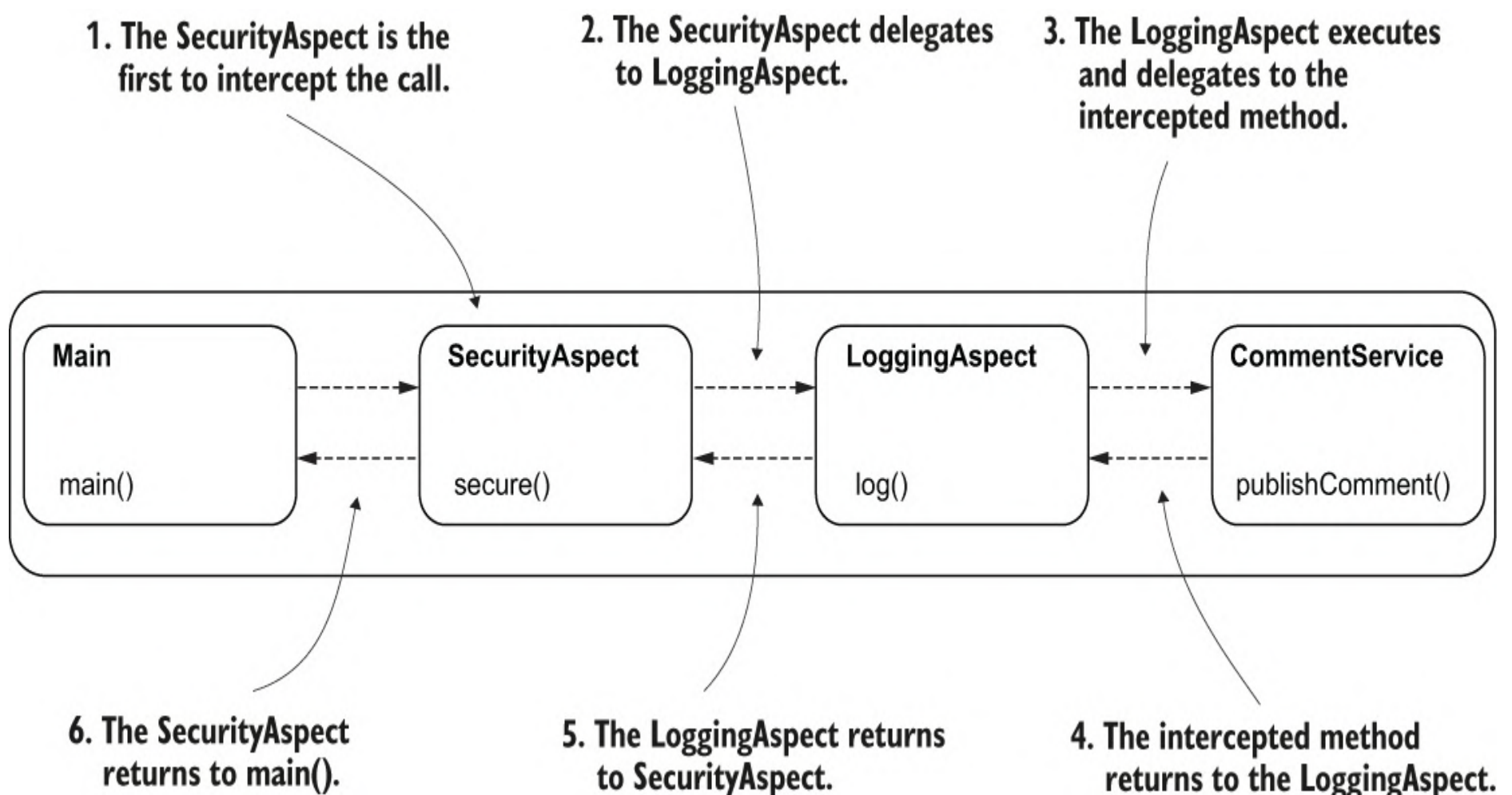
Figure 6.16 The execution flow after changing the order of the aspects. The SecurityAspect was first to intercept the method call and delegates further in the execution chain to the LoggingAspect, which further delegates the call to the intercepted method. The intercepted method returns to the LoggingAspect, which returns further to the SecurityAspect.
