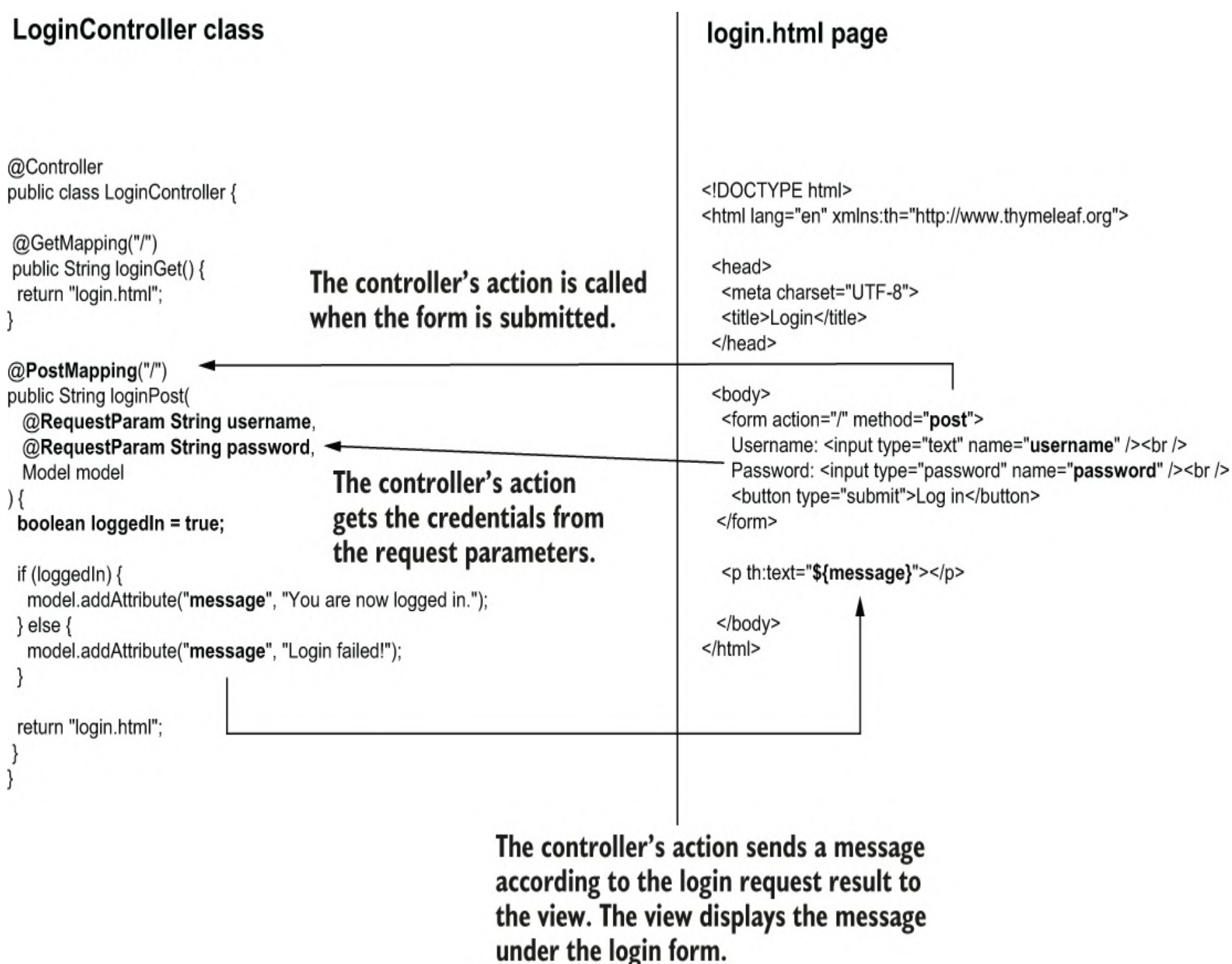
Figure 9.5 The dispatcher servlet calls the controller's action when someone submits the HTML login
