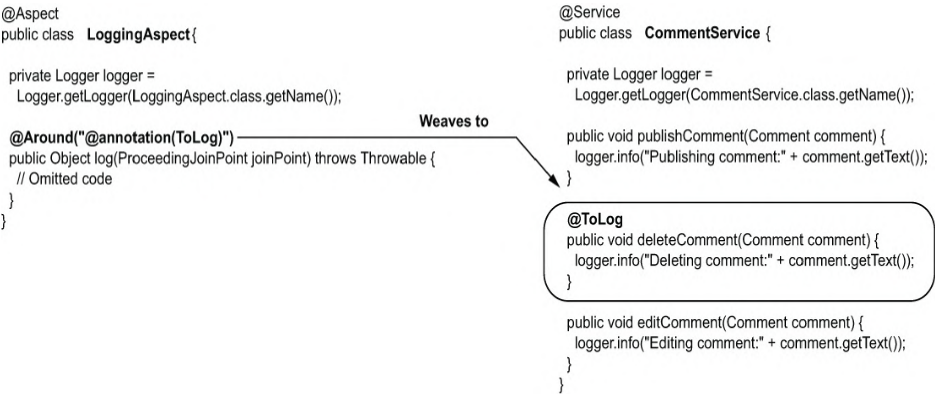
Figure 6.13 Using an AspectJ pointcut expression, we weave the aspect logic to any method annotated
