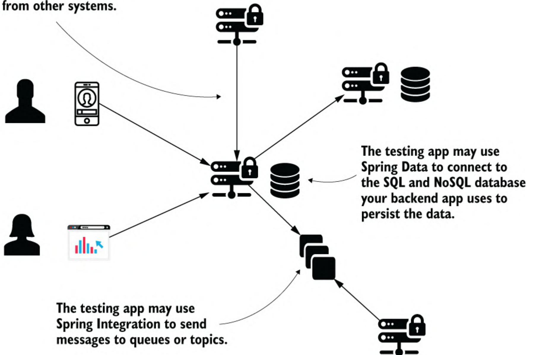
Figure 1.8 A testing app might need to connect to databases or communicate with other systems or the tested system. The developers can use components of the Spring ecosystem to simplify the implementations of these functionalities.
