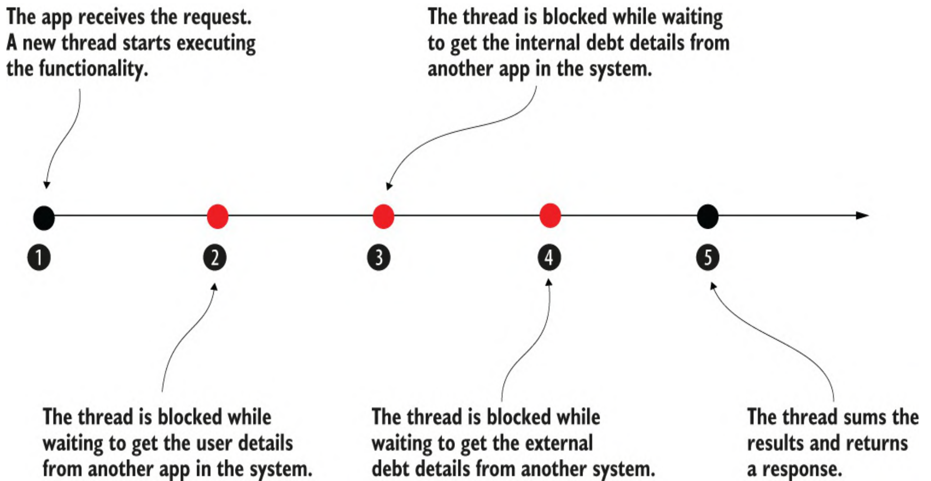
Figure 11.8 The execution of the scenario functionality from the thread point of view. The arrow represents the timeline of the thread. Some of the steps cause details to block the thread, which needs to wait for the task to finish before proceeding.
