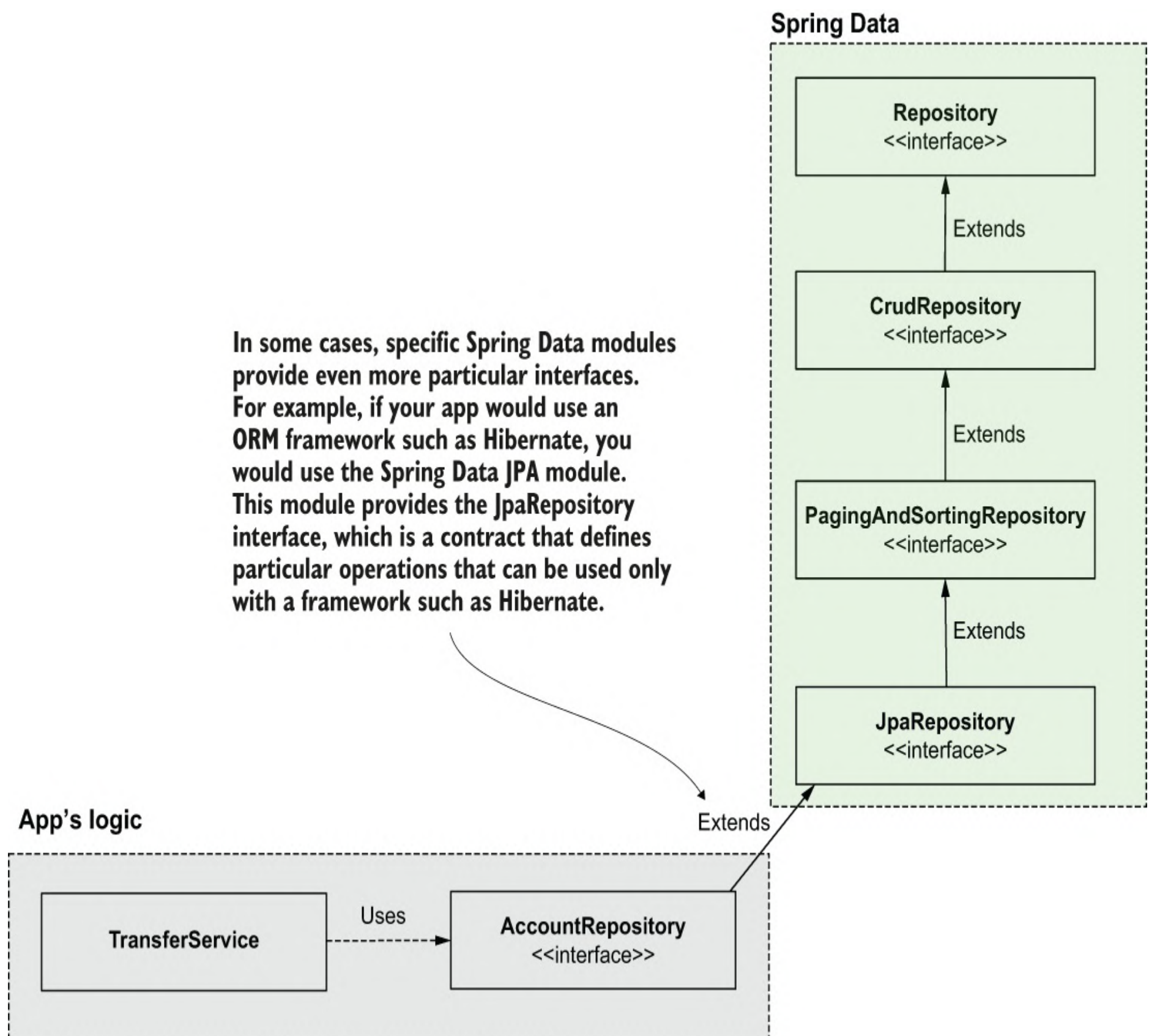
Figure 14.10 Different Spring Data modules might provide other, more particular contracts. For example, if you use an ORM framework such as Hibernate (which implements the JPA) with Spring Data, you can extend the JpaRepository interface, which is a more particular contract that provides operations applicable only when using a JPA implementation, such as Hibernate.
