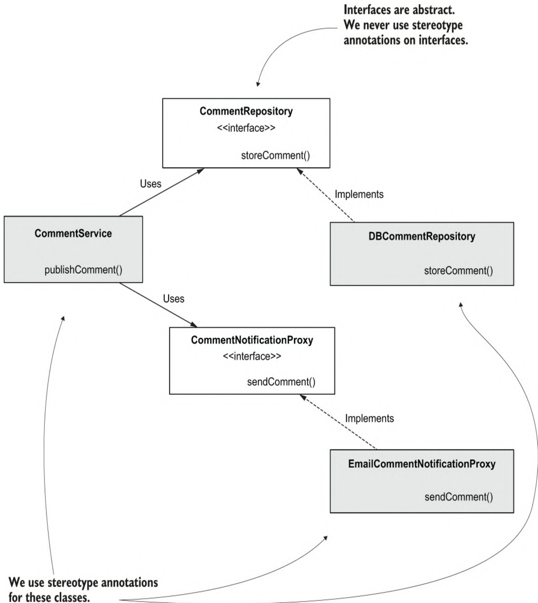
Figure 4.8 The classes we'll mark with the @Component stereotype annotation are shaded gray. When the context is loaded, Spring creates instances of these classes and adds them to its context.
