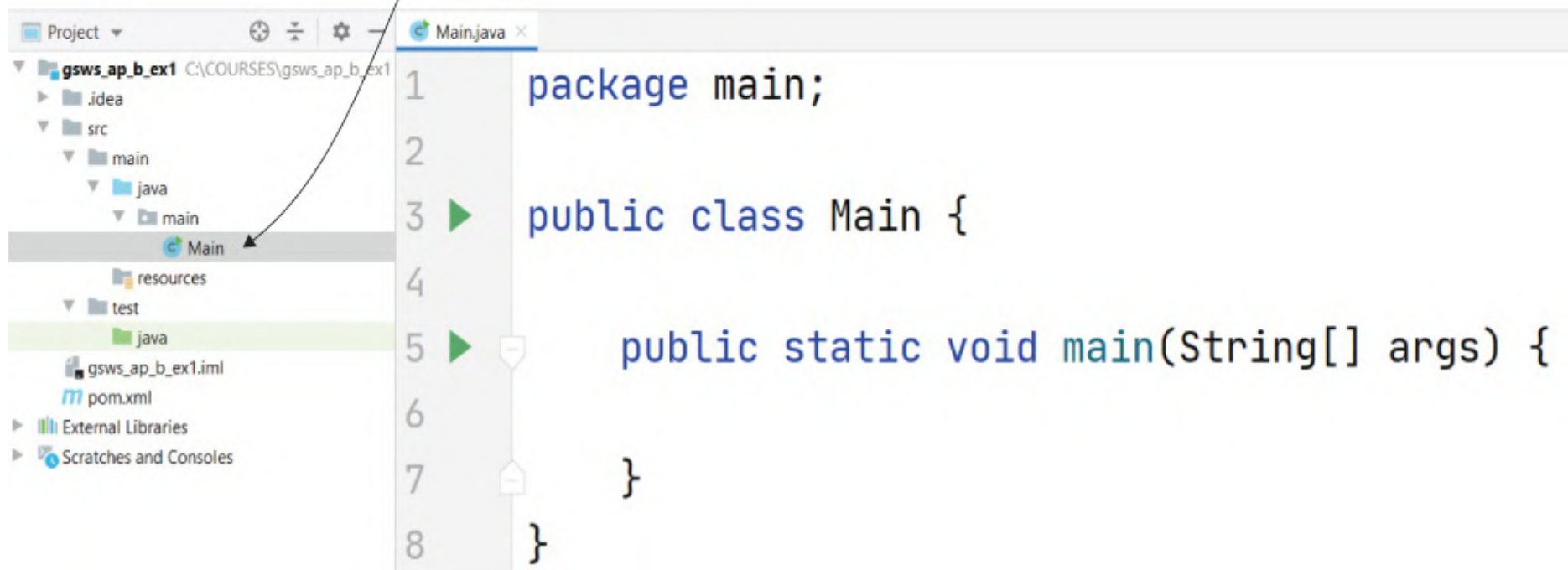
Figure 2.4 Inside the “java” folder, you create the usual Java packages and classes of your application. These are the classes that define the whole logic of your app and make use of the dependencies you provide.
