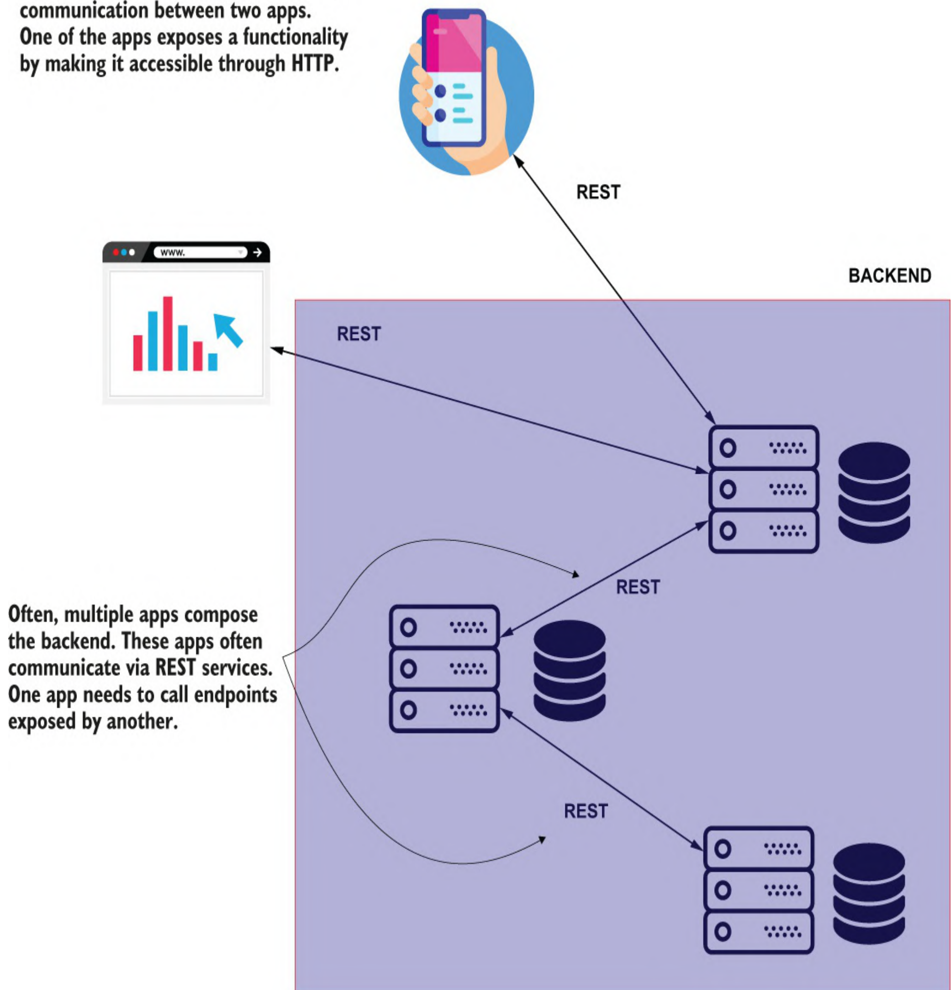
Figure 11.1 Often, a backend app needs to act as a client for another backend app, and calls exposed REST endpoints to work with specific data.
