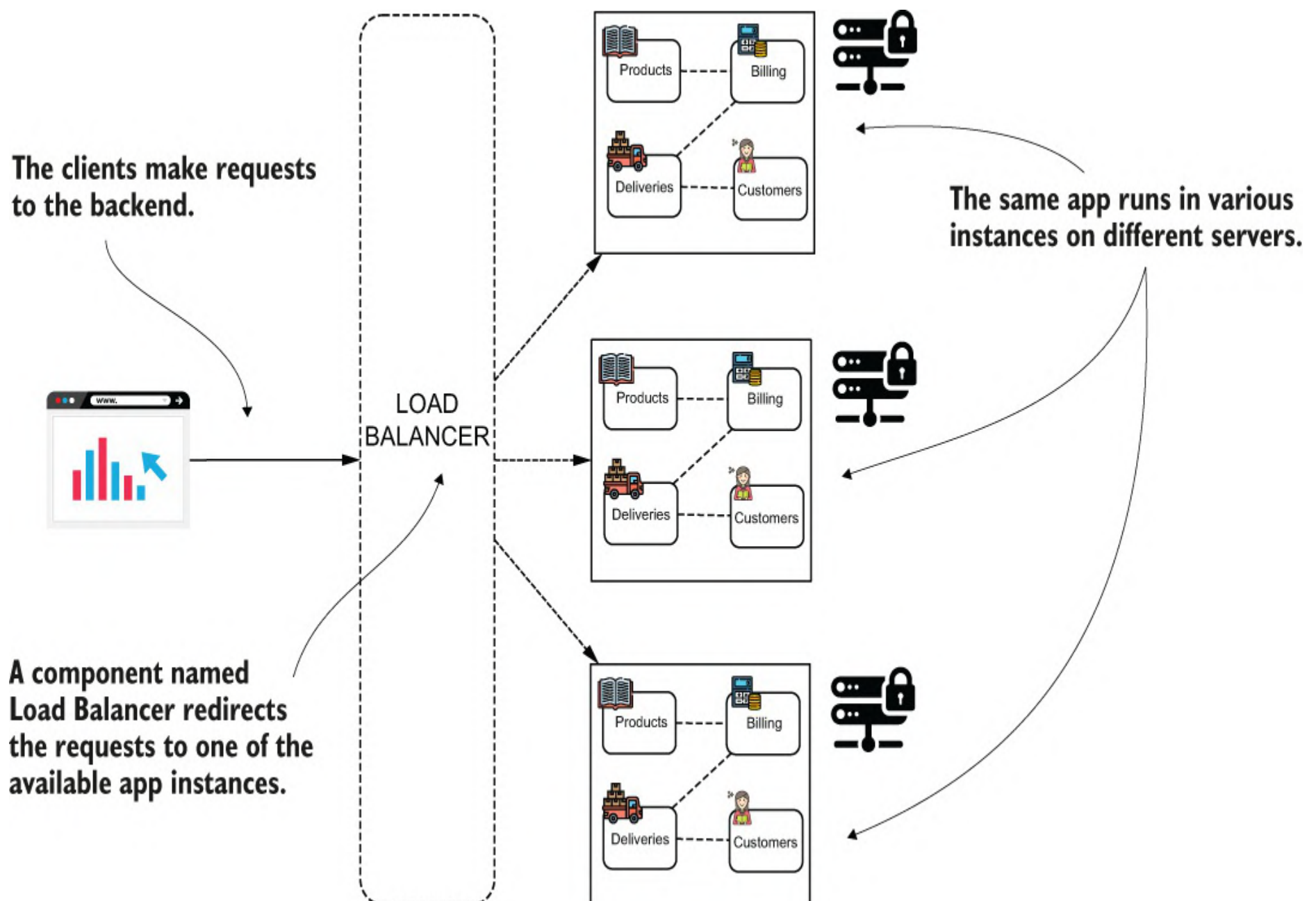
Figure A.3 Horizontal scaling. Running the same instance multiple times enables us to use more resources and serve more client requests.
