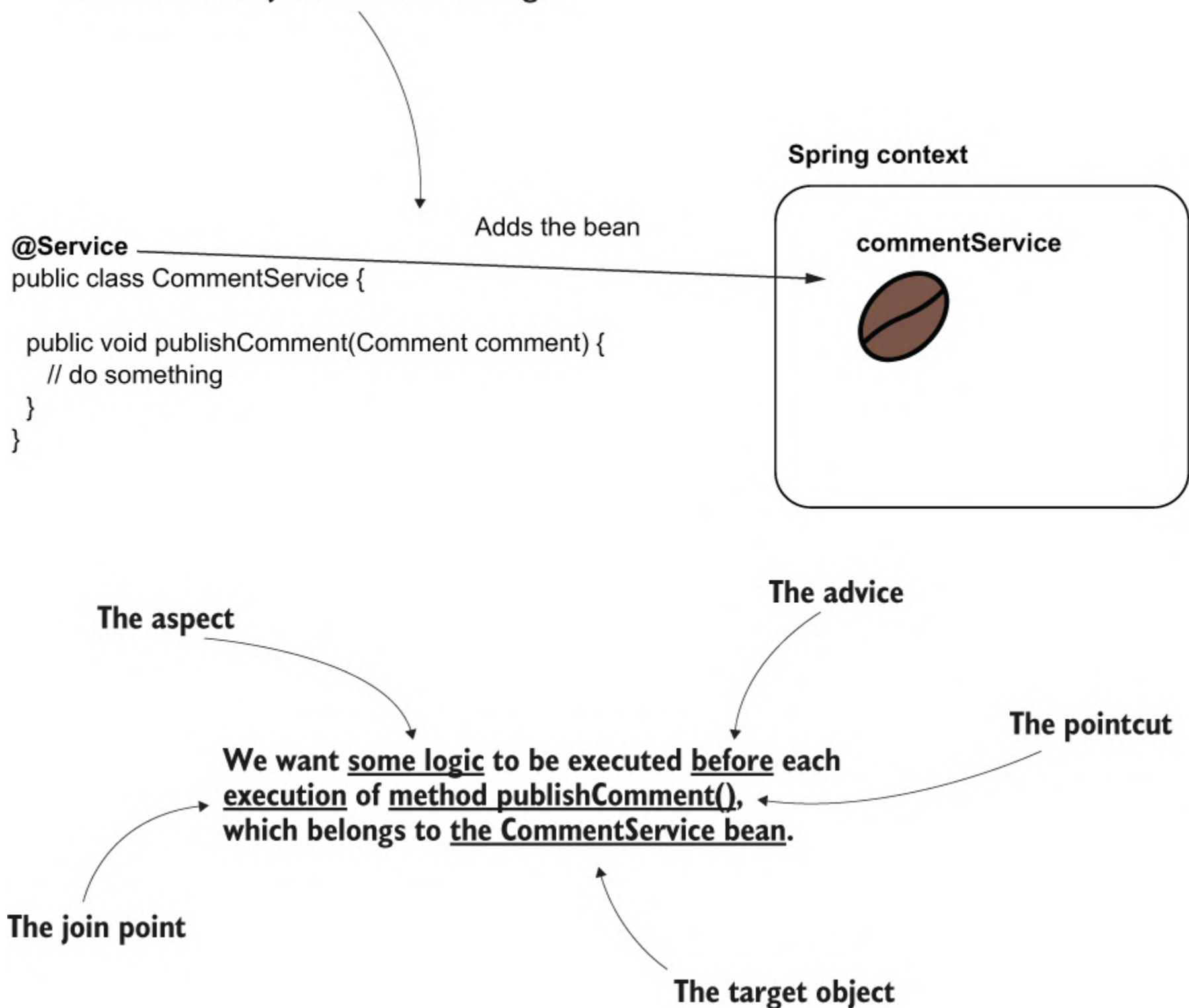
Figure 6.2 The aspect terminology. Spring executes some logic (the aspect) when someone calls a specific method (the pointcut). We need to specify when the logic is executed according to the pointcut (e.g., before). The when is the advice. For Spring to intercept the method, the object that defines the intercepted method needs to be a bean in the Spring context. So, the bean becomes the target object of the aspect.
