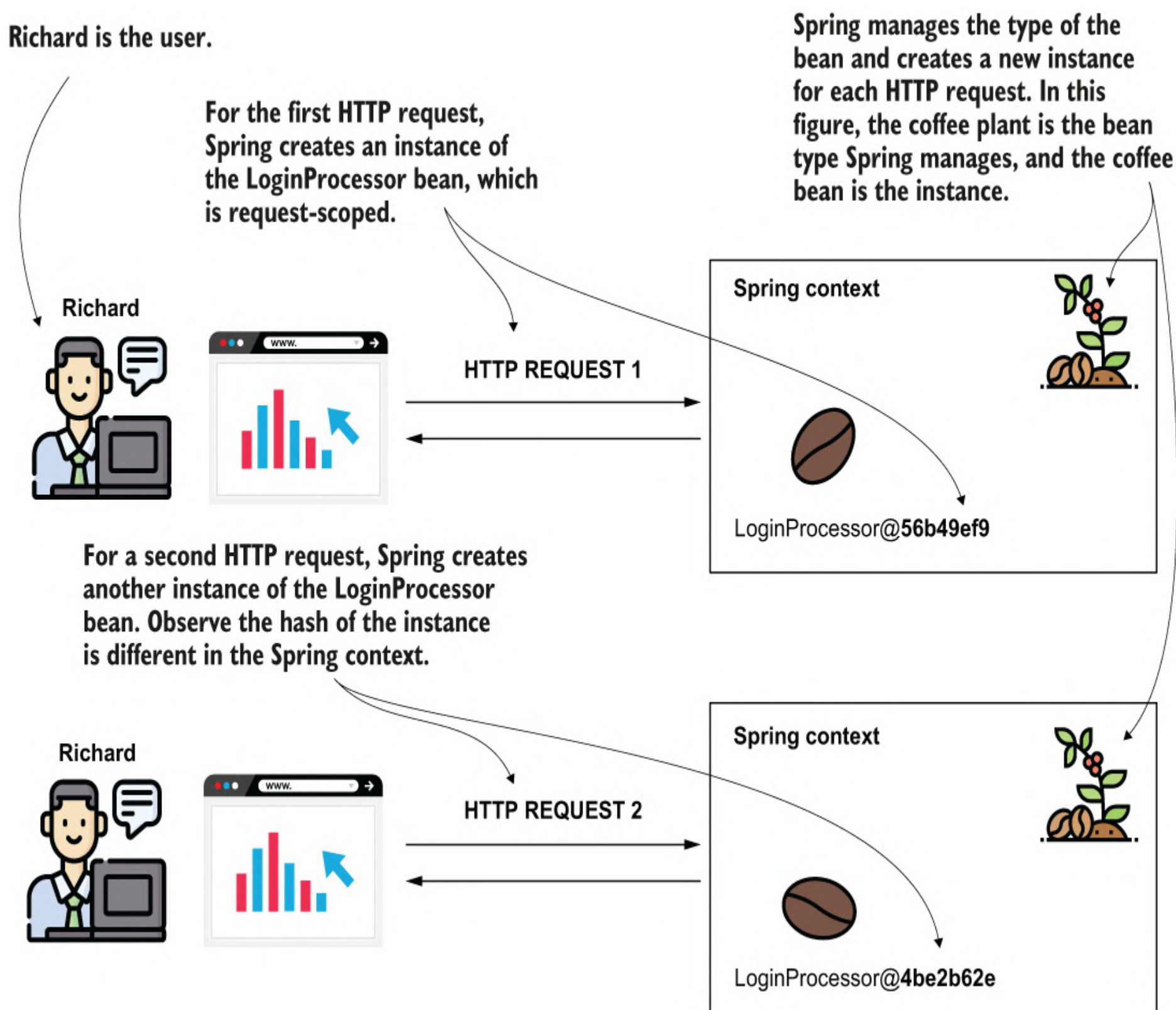
Figure 9.2 For every HTTP request, Spring provides a new instance for the request-scoped bean. When using a request-scoped bean, you can be sure the data you add on the bean is available only on the HTTP request that created the bean. Spring manages the bean type (the plant) and uses it to get instances (coffee beans) for each new request.
