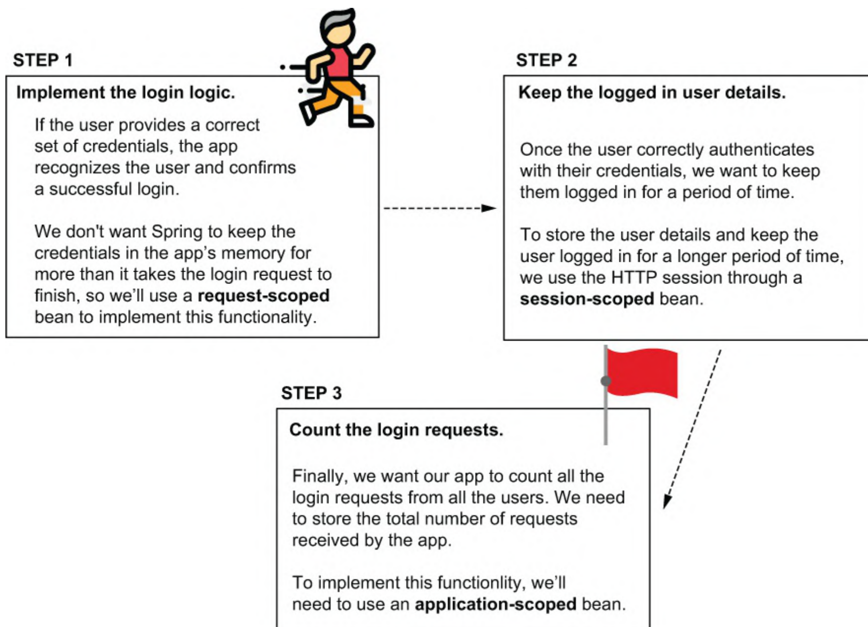
Figure 9.1 We'll implement the login functionality in three steps. For each step we implement, we'll need to use a different bean scope. In section 9.1, we'll use a request-scoped bean to implement the login logic without risking storing the credentials for longer than the login request. We'll then decide what details we need to store for the authenticated user in a session-scoped bean. Finally, we'll implement a feature to count all the login requests, and we'll use an application-scoped bean to keep the number.
