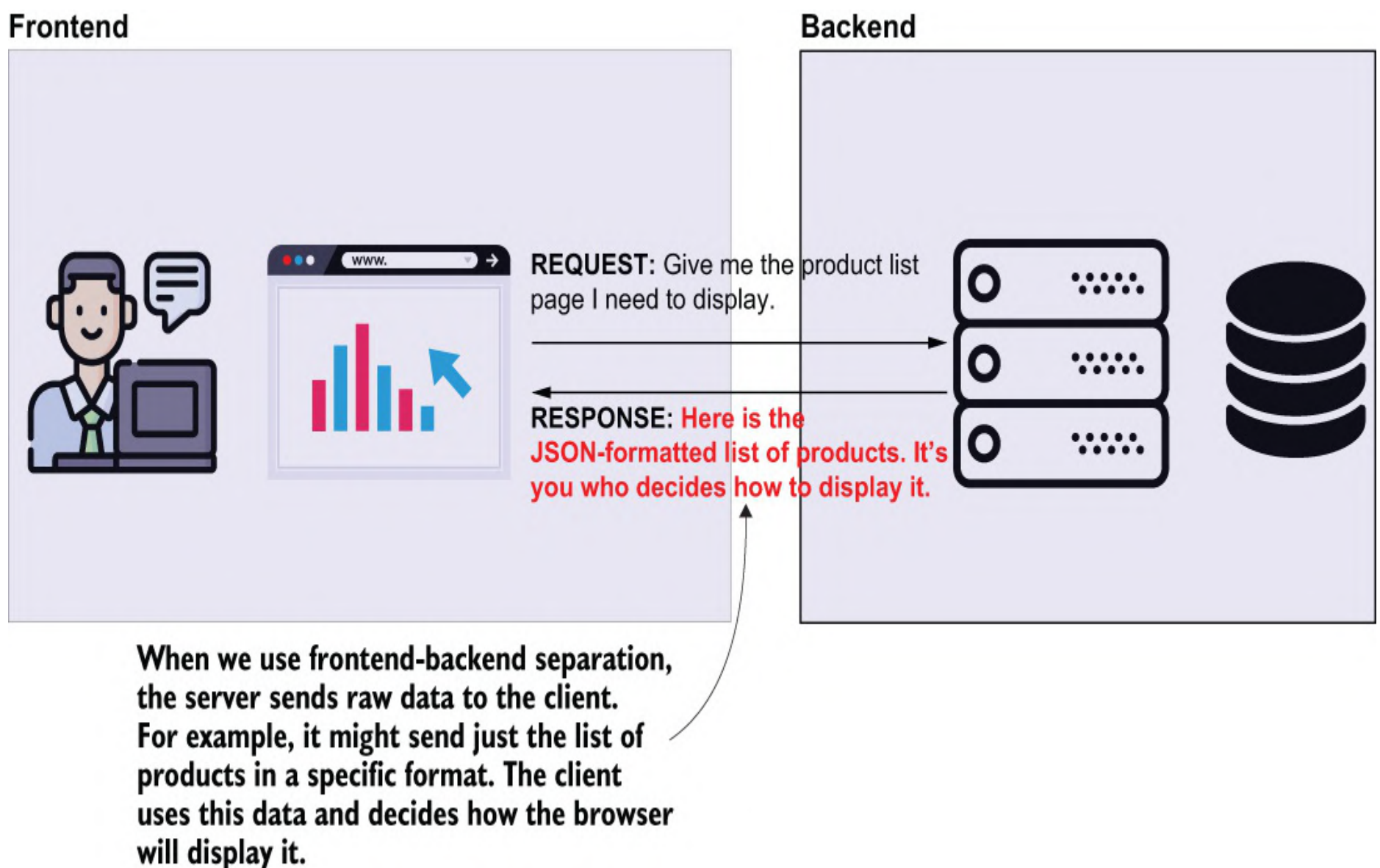
Figure 7.5 Using frontend-backend separation. The server doesn't respond with the exact data that needs to be displayed by the browser. The backend sends the data to the client but doesn't tell the browser how to display this data or what to do with it. The backend now only sends raw data (usually in an easily parsable format like JSON or XML). The browser executes a frontend app that takes the server's raw response and processes it to display the data.
