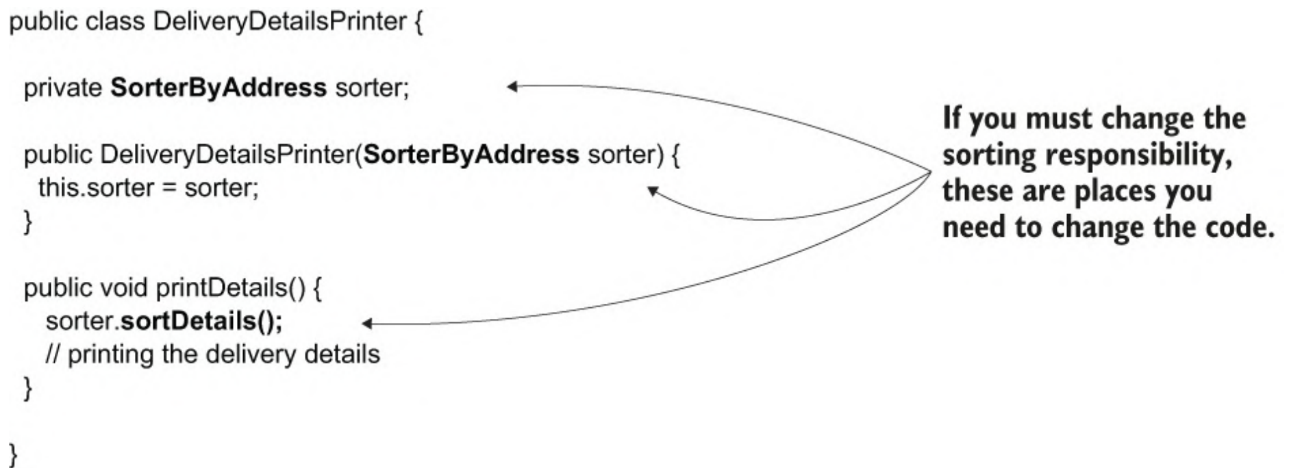
Figure 4.2 Because the two objects are strongly coupled, if you want to change the sorting responsibility, you also need to change the object using this responsibility. A better design would allow you to change the sorting responsibility without changing the object that uses the responsibility.
