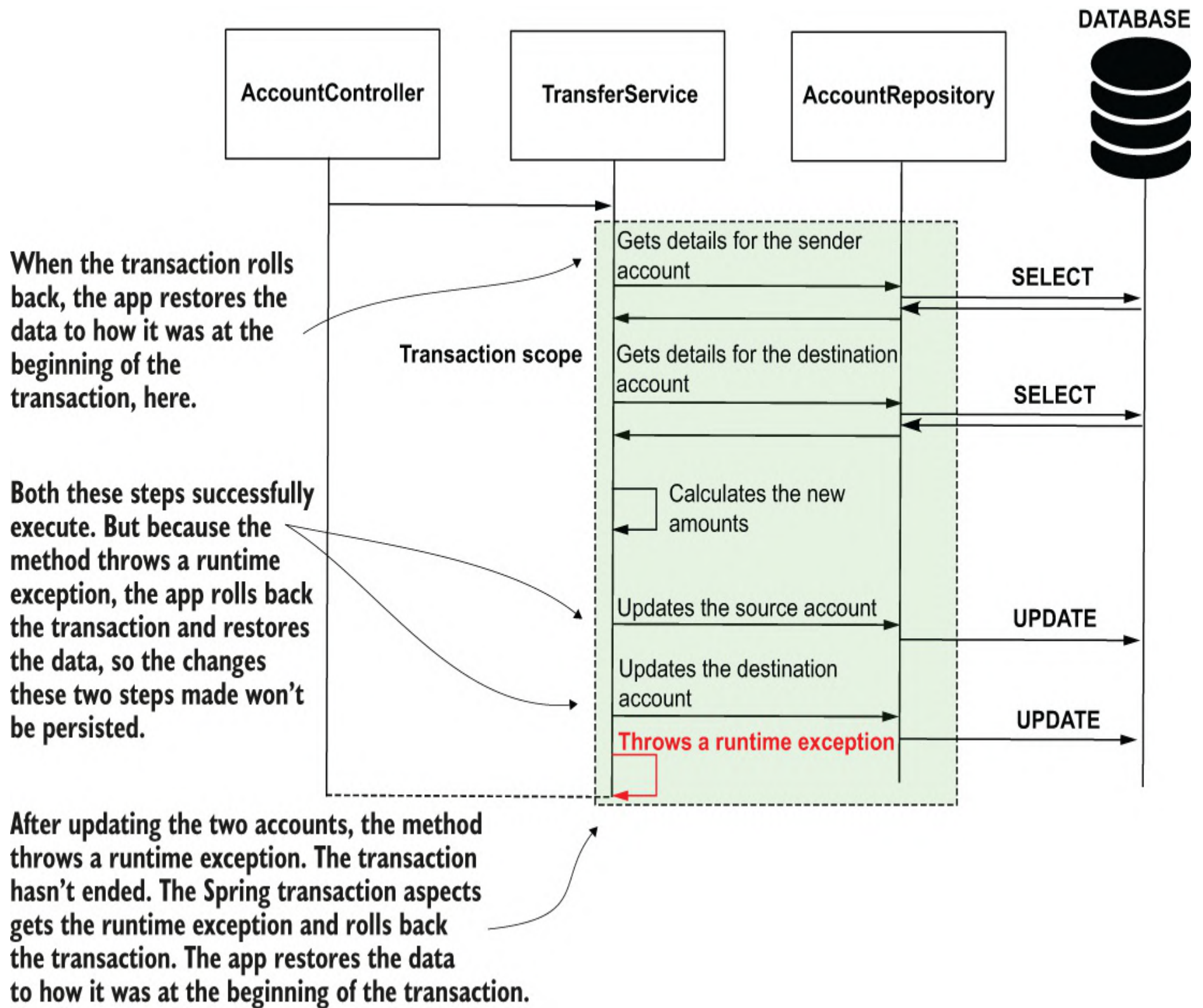
Figure 13.8 When the method throws a runtime exception, Spring rolls back the transaction. All the successful changes made on the data are not persisted. The app restores the data to how it was when the transaction started.
