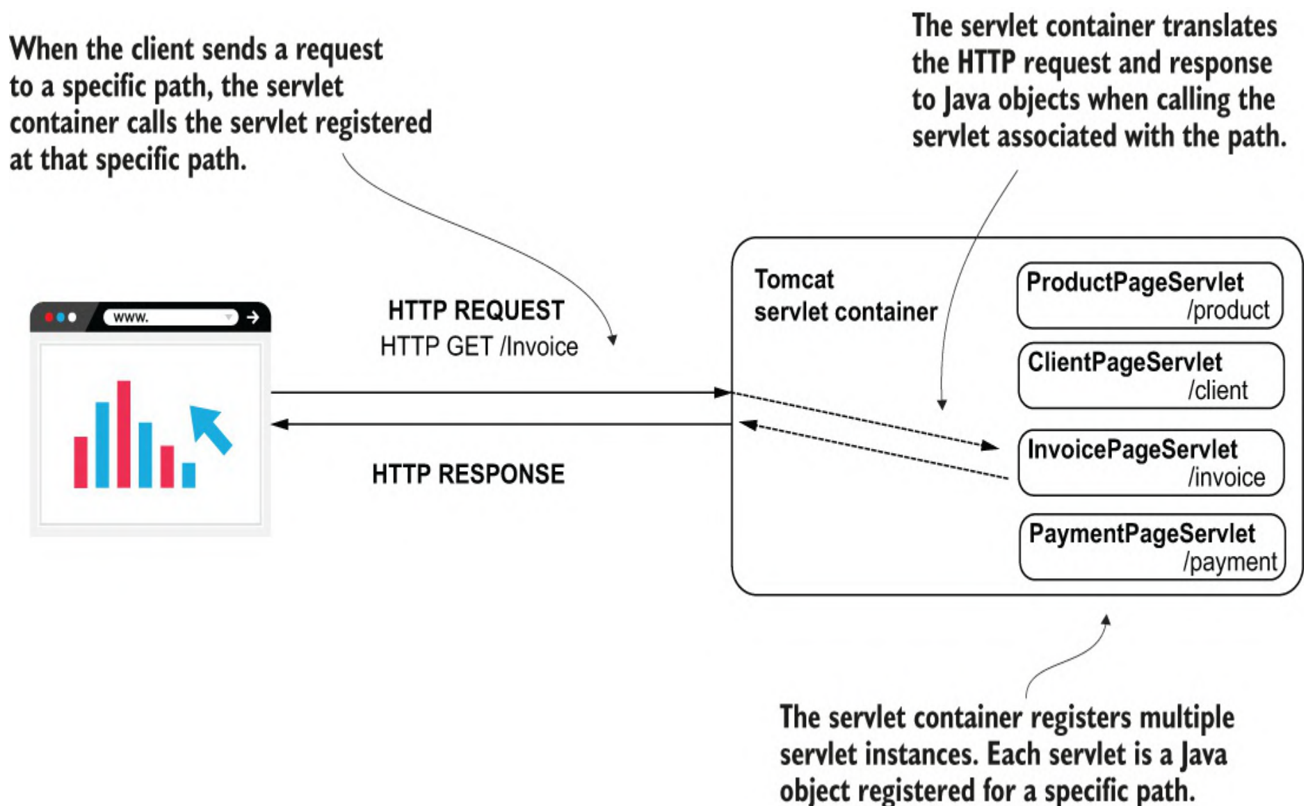
Figure 7.7 The servlet container (Tomcat) registers multiple servlet instances. Each servlet is associated with a path. When the client sends a request, Tomcat calls a method of the servlet associated with the path the client requested. The servlet gets the values on the request and builds the response that Tomcat sends back to the client.
