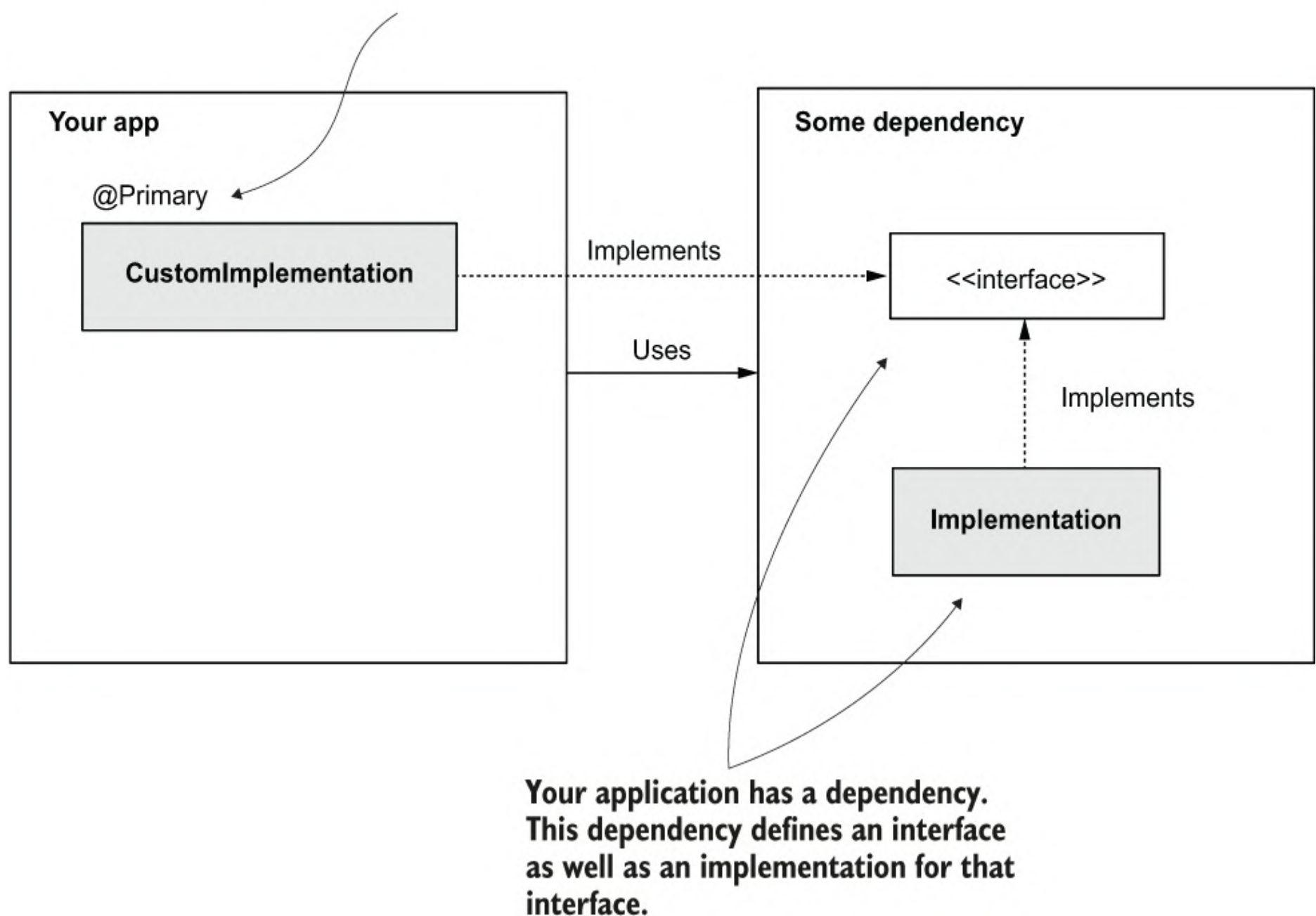
Figure 4.10 Sometimes you use dependencies that already provide implementations for specific interfaces. When you need to have custom implementations of those interfaces, you can use @Primary to mark your implementation as a default for DI. This way, Spring knows to inject the implementation you
