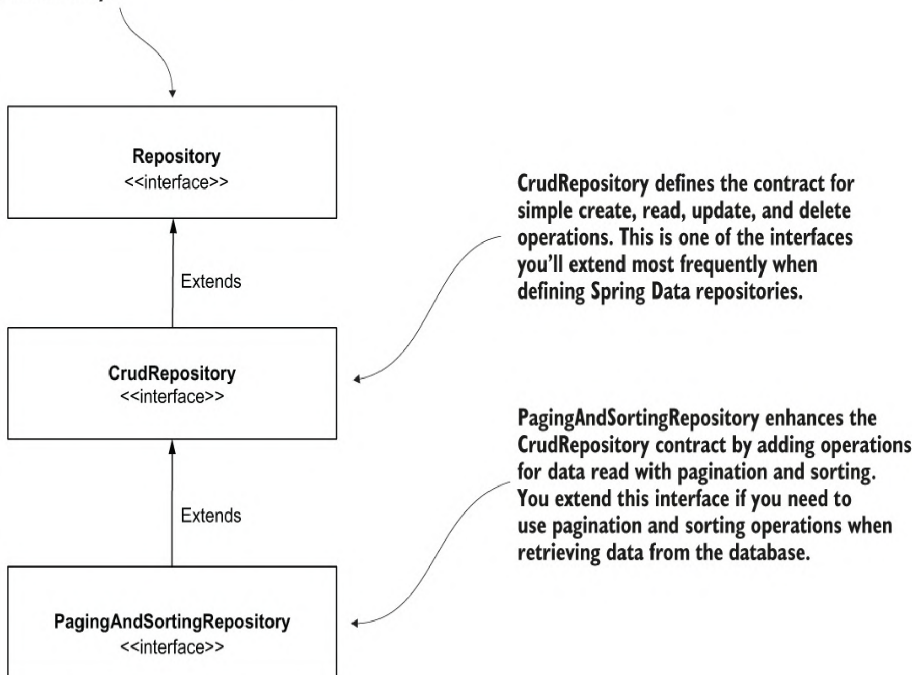
Figure 14.6 To implement your app's repositories using Spring Data, you extend specific interfaces. The main interfaces that represent Spring Data contracts are Repository , CrudRepository , and PagingAndSortingRepository . You extend one of these contracts to implement your app's persistence capabilities.
