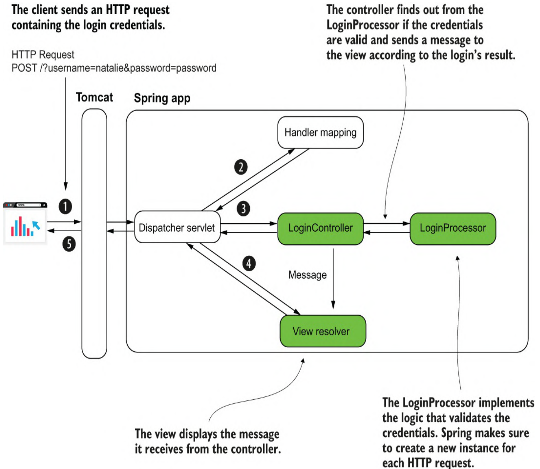
Figure 9.6 The LoginProcessor bean is request-scoped. Spring makes sure to create a new instance for each HTTP request. The bean implements the login logic. The controller calls a method it implements. The method returns true if the credentials are valid and false otherwise. Based on the value the LoginProcessor returns, the LoginController sends the right message to the view.
