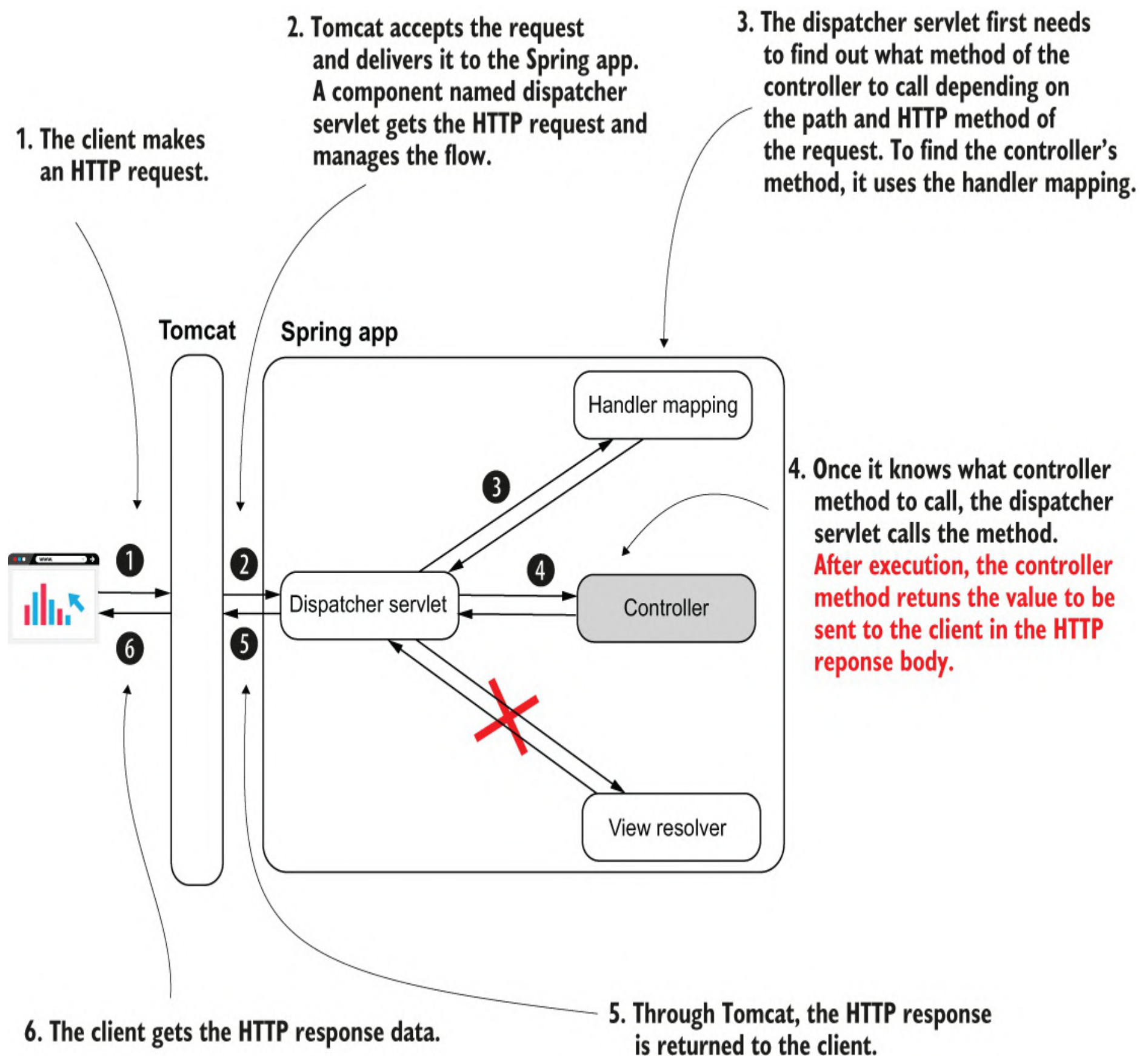
Figure 10.2 When implementing REST endpoints, the Spring MVC flow changes. The app no longer needs a view resolver because the client needs the data returned by the controller's action directly. Once the controller's action completes, the dispatcher servlet returns the HTTP response without rendering any view.
