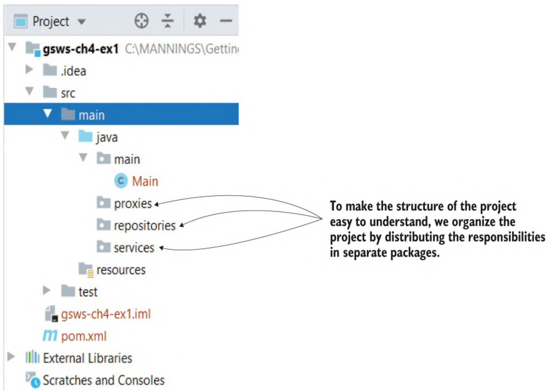
Figure 4.7 The project structure. We declare a separate package for each responsibility to make the structure of the project easy to read and understand.
