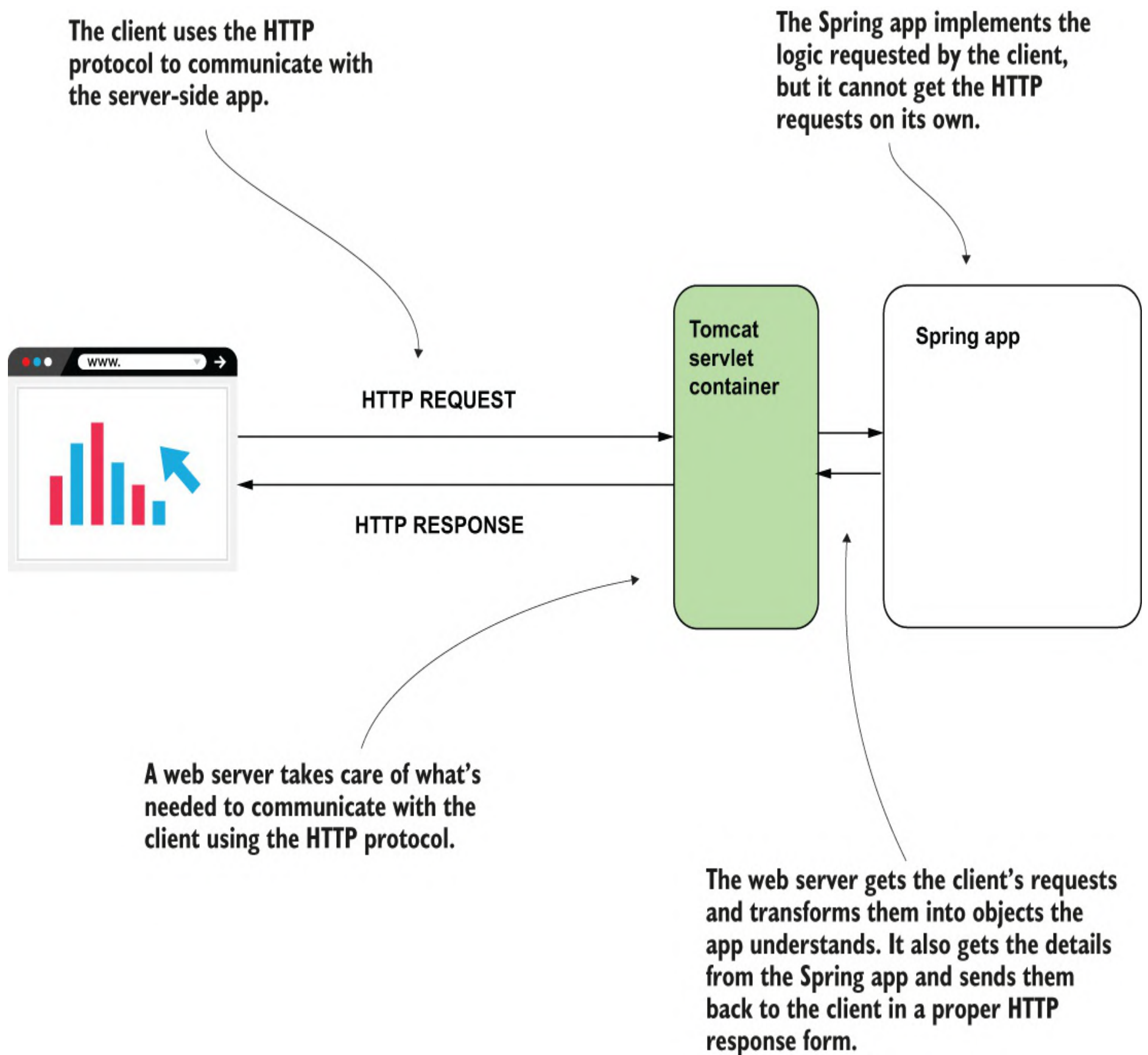
Figure 7.6 A servlet container (e.g., Tomcat) speaks HTTP. It translates the HTTP request to our Spring app and the app's response into an HTTP response. This way, we don't need to care about the protocol used for communication on the network, as we simply write everything as Java objects and methods.
